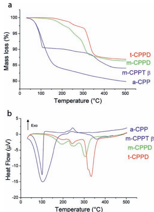
Figure 5. (a) TGA and (b) DTA curves of the pure hydrated calcium pyrophosphate phases synthesised.
