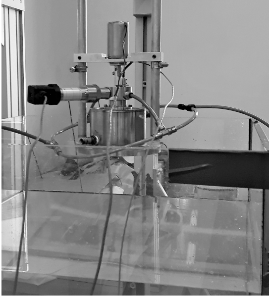
Figure 2. JaLaD experimental Set-up.
