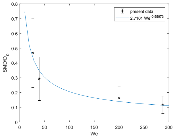
Figure 6. Sauter Mean Diameter as a function of Weber number. The blue curve is a power-law fitting of the data
