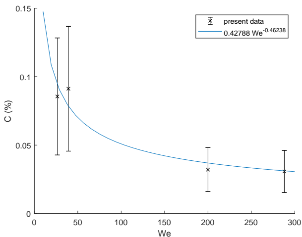
Figure 7. Kinetic to surface energy conversion ratio C as a function of Weber number. The blue curve is a power-law fitting of the data
