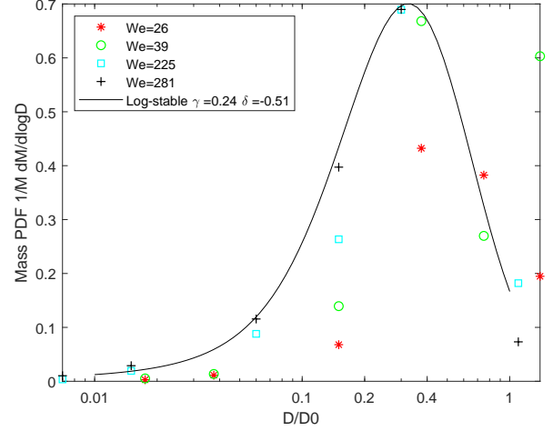
Figure 5. Mass Distribution
