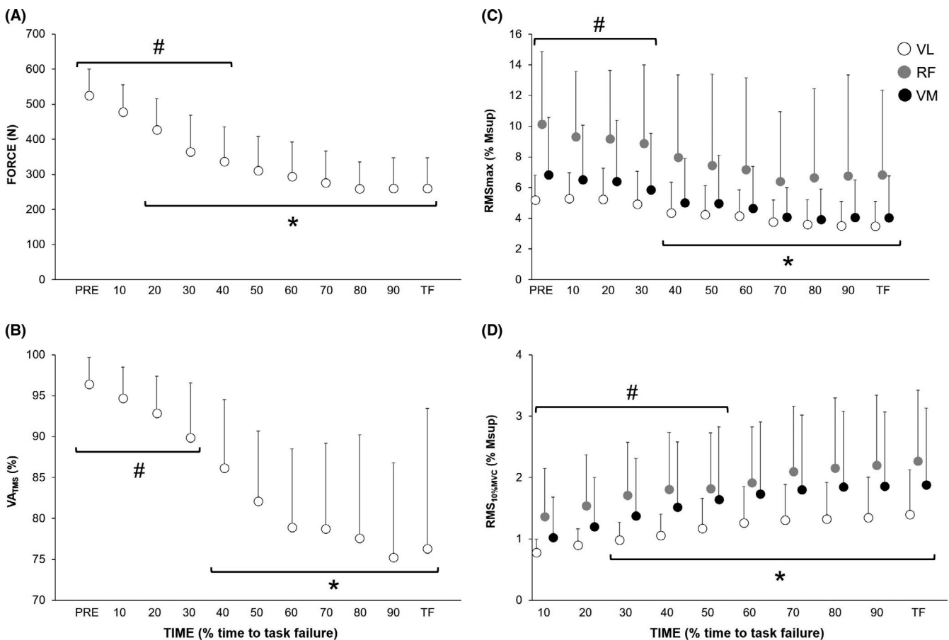
FIGURE 3 Changes in knee extensors maximal voluntary contraction (MVC) isometric force (A), voluntary activation ( VA_{TMS} ; B), and maximal root-mean-square EMG ( RMS_{MAX} ; C) during (10%, 20%, 30%, 40%, 50%, 60%, 70%, 80%, and 90% of the time to task failure) and immediately at task failure (TF, performed as an extension of the prolonged submaximal voluntary contraction). Panel D displays the root-mean-square EMG recorded 500 ms before the brief MVCs during the sustained submaximal voluntary contraction. Data are presented as mean \pm SD. Significantly different from PRE: * P < .05 . Significantly different from TF: # P < .05
