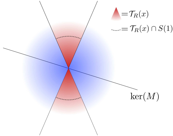
Fig. 1 A representation of recovery guarantees based on descent cones of a convex function. Recovery of x \in \Sigma fails if \ker(M) intersects \mathcal{T}_R(x) non trivially. The bigger is the descent cone (red) the more likely recovery will fail. The bigger the space left by the descent cone (blue), the more likely recovery will succeed
