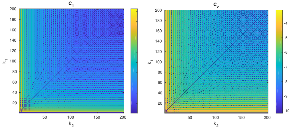
Fig. 3 Then quantities \log_{10}(C_1(k_1, k_2)) := \log_{10}\left(\left|1 - \frac{\langle w^*, w_0 \rangle}{\|w^*\|_2 \|w_0\|_2}\right|\right) (left) and \log_{10}(C_2(k_1, k_2)) := \log_{10}(|\delta_{\Sigma}^{\text{nec}}(\|\cdot\|_{w^*}) - \delta_{\Sigma}^{\text{nec}}(\|\cdot\|_{w_0})|) (right) where w^* = (w_1^*, w_2^*) is obtained from Theorem 7 and w_0 = (1/\sqrt{k_1}, 1/\sqrt{k_2}) for different k_1, k_2 \geq 2 .
