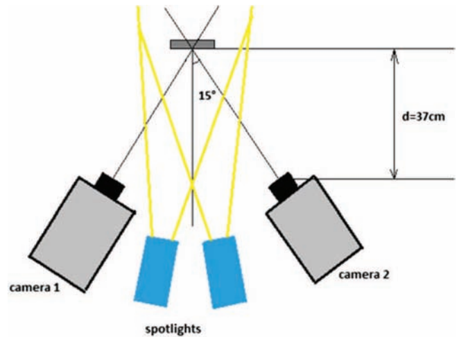
Figure 4: Stereo-DIC setup
