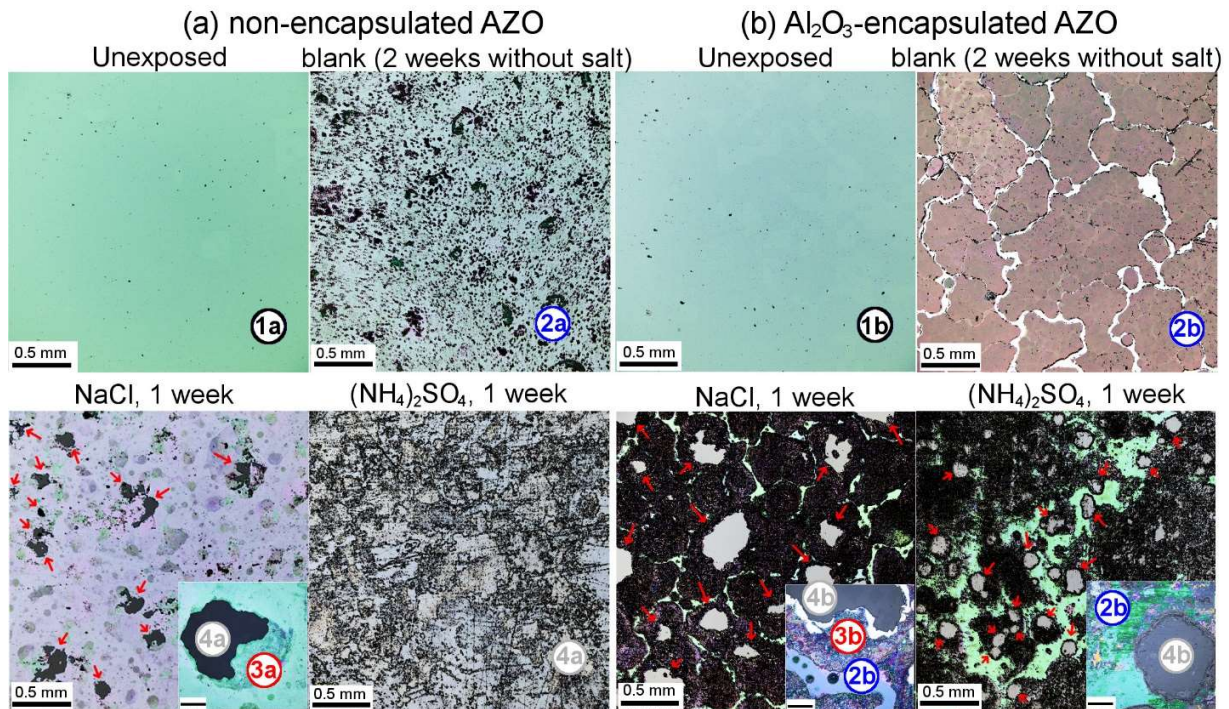
Fig. 5. Confocal optical microscope images of (a) non-encapsulated and (b) Al 2 O 3 -encapsulated AZO samples. High resolution optical images are shown in insets (scale bar 50 \mu m). Red arrows indicate locally dissolved areas in which the height is approximately 340 nm lower than in the surrounding areas. Exposure conditions (cycling time and salt used for the aerosol deposit) are indicated.
