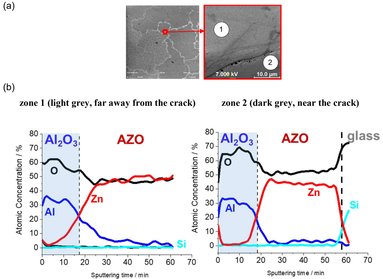
Fig. 7. (a) Secondary electron images of blank \text{Al}_2\text{O}_3 -encapsulated AZO sample after two weeks' exposure without salt and (b) AES depth profiles recorded in zones 1 and 2 shown in (a). Zone 1 is far away from the crack and zone 2 is near the crack.
