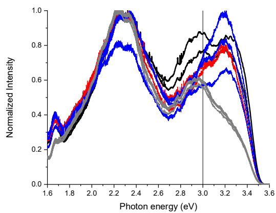
Figure S1: Examples of room temperature PL spectra of (a) as deposited non-encapsulated and \text{Al}_2\text{O}_3 -encapsulated AZO samples as indicated and (b) non-encapsulated AZO exposed to different climatic chamber exposure conditions (unexposed samples in black, exposed without salt in grey, exposed with NaCl in blue and red). Vertical lines show the position of 3 eV band associated with doping.
