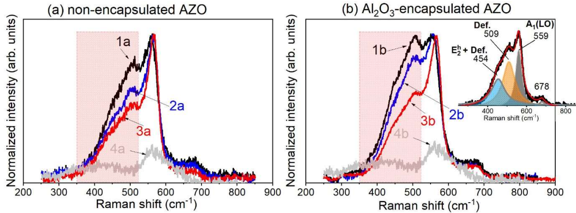
Fig. 6. Representative Raman spectra of different zones of (a) non-encapsulated and (b) \text{Al}_2\text{O}_3 -encapsulated AZO thin films exposed to different climatic test conditions. The labels reflect the zones of different types, shown in Fig. 5. Spectra 1-3 are normalized by the A_1(\text{LO}) band of ZnO. Spectra 4a and 4b coincide with the Raman spectra of the glass substrate. The inset in (b) illustrates an example of the peak fitting performed by 3 Lorentz curves.
