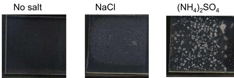
Figure S5: Example of photographs, showing the surface appearance of (a) non-encapsulated and (b) \text{Al}_2\text{O}_3 -encapsulated samples after one week of the test with and without salt deposition (as indicated). The sample size is 3.0 \times 3.0 \text{ cm}^2 for (a) and 2.5 \times 2.5 \text{ cm}^2 for (b).
