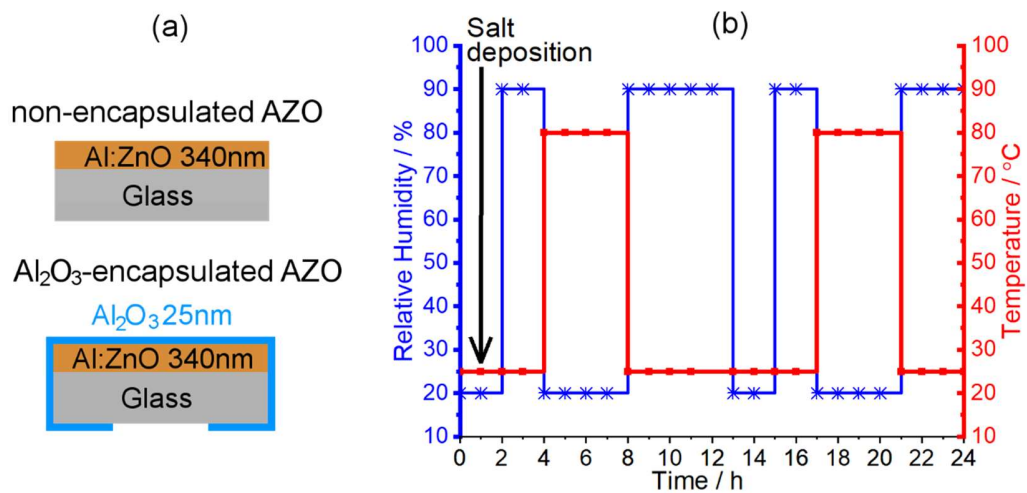
Fig. 1. Schematics of (a) sample configurations and (b) one-day (24 h) cycle of new climatic test. The test duration was 7 or 14 days. In both cases, salt was deposited only during the first five days.
