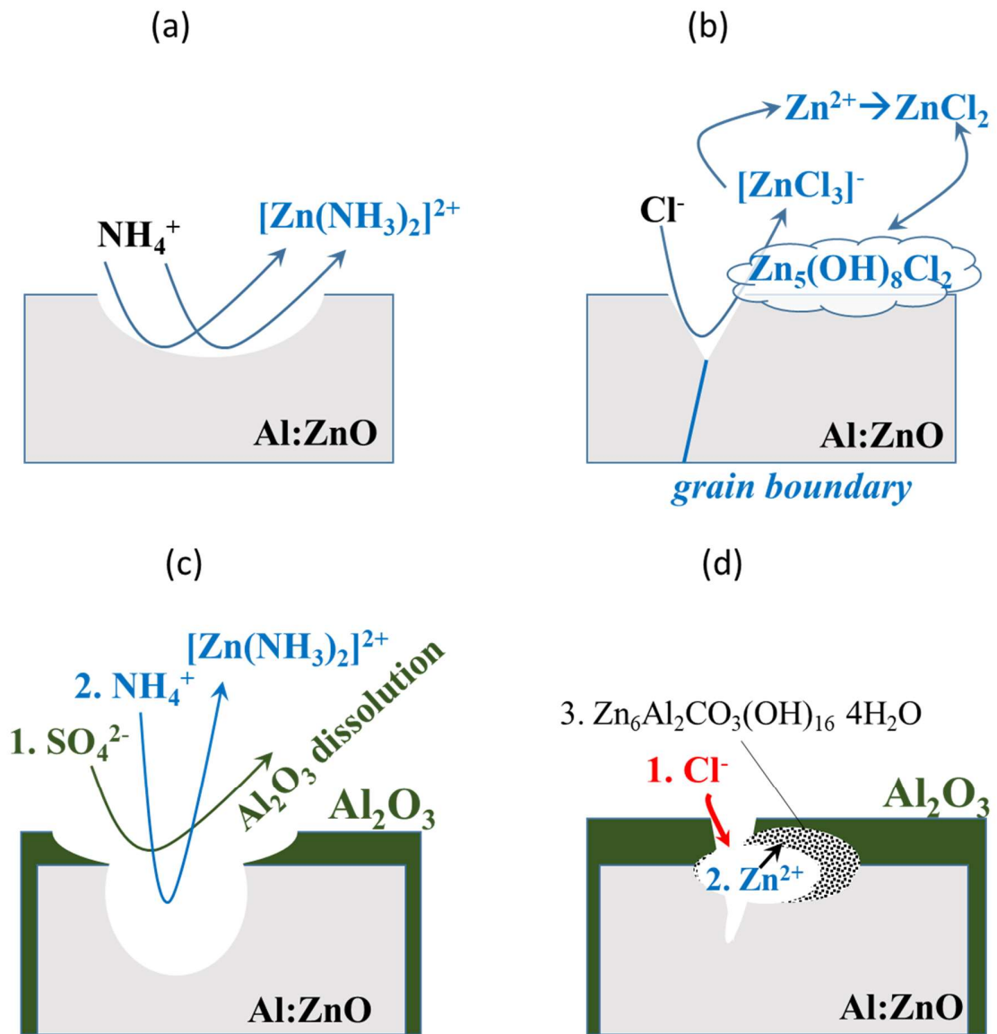
Fig. 8 Chemical degradation of non-encapsulated and \text{Al}_2\text{O}_3 -encapsulated Al-doped ZnO (Al:ZnO) layers on glass exposed in a climatic test to aerosols of NaCl or (\text{NH}_4)_2\text{SO}_4 . (a) Dissolution of non-encapsulated AZO induced by deposited (\text{NH}_4)_2\text{SO}_4 via soluble Zn complexes with \text{NH}_3 . (b) Local dissolution of non-encapsulated AZO induced by deposited NaCl via soluble Zn complexes with \text{Cl}^- . (c) Step 1 shows slow pit initiation with rapid pit growth of \text{Al}_2\text{O}_3 in the presence of sulphate, followed by step 2 where AZO dissolution by ammonium in areas of dissolved \text{Al}_2\text{O}_3 . (d) Step 1 shows quick pit initiation in \text{Al}_2\text{O}_3 by chloride, followed by step 2 where AZO dissolution in the confined zone and step 3 where \text{Al}_2\text{O}_3 is transformed into \text{Zn}_6\text{Al}_2\text{CO}_3(\text{OH})_{16} \cdot 4\text{H}_2\text{O} (LDH).
