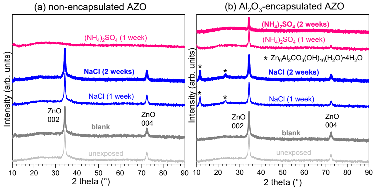
Fig. 4. Bragg-Brentano XRD of (a) non-encapsulated AZO and (b) \text{Al}_2\text{O}_3 -encapsulated AZO samples after climatic test. The test duration is indicated for the samples exposed with NaCl or (\text{NH}_4)_2\text{SO}_4 , blank sample was exposed for two weeks without salt. The reference patterns are ZnO (JCPDS 00-036-1451) and \text{Zn}_6\text{Al}_2\text{CO}_3(\text{OH})_{16}(\text{H}_2\text{O})\cdot 4\text{H}_2\text{O} (JCPDS 00-038-0486).
