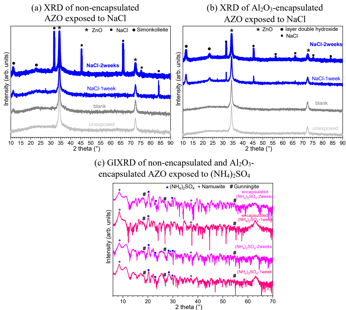
Figure S2: XRD of (a) non-encapsulated and (b) Al 2 O 3 -encapsulated AZO exposed to NaCl, and (c) GIXRD of both non-encapsulated and Al 2 O 3 -encapsulated AZO exposed to (NH 4 ) 2 SO 4 . All the samples analysed without washing after the exposures.
