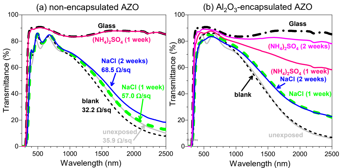
Fig. 2. Optical transmittance of (a) non-encapsulated AZO and (b) \text{Al}_2\text{O}_3 encapsulated AZO samples. Results for unexposed, blank (two weeks' exposure without salt), and exposed with NaCl or (\text{NH}_4)_2\text{SO}_4 deposits for 1 and 2 weeks are shown, as indicated.
