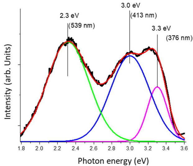
Fig. 3. Example of room temperature photoluminescence spectrum of unexposed AZO.
