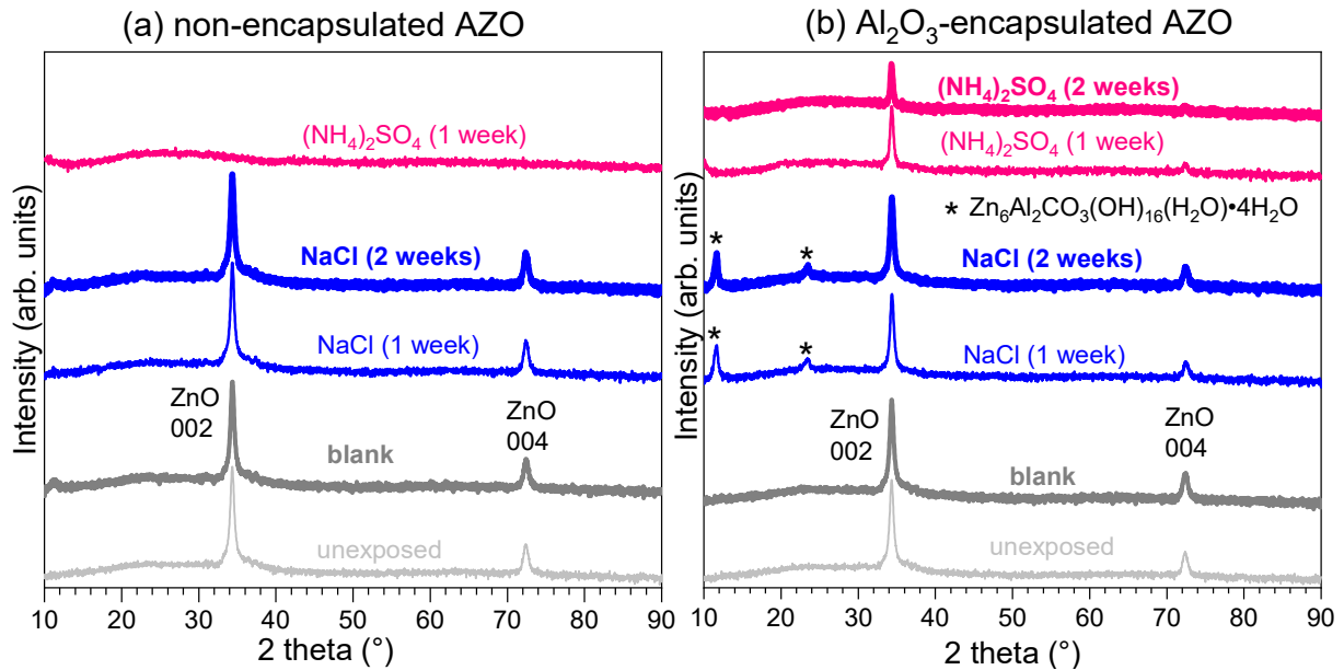
Fig. 4. Bragg-Brentano XRD of (a) non-encapsulated AZO and (b) Al 2 O 3 -encapsulated AZO samples after climatic test. The test duration is indicated for the samples exposed with NaCl or (NH 4 ) 2 SO 4 , blank sample was exposed for two weeks without salt. The reference patterns are ZnO (JCPDS 00-036-1451) and Zn 6 Al 2 CO 3 (OH) 16 (H 2 O)·4H 2 O (JCPDS 00-038-0486).
