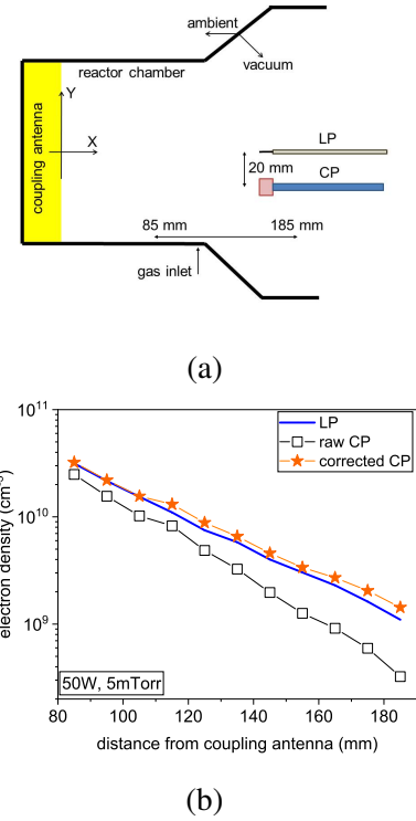
Figure 2: (a) Measurement setup. (b) Longitudinal profile along plasma expansion.
