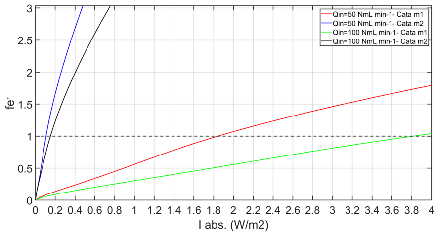
Figure 8 Representation of the fe' criterion vs I_{abs} - C_{in}=10 ppm - \psi = 0.98/2 – PolyActive membrane
