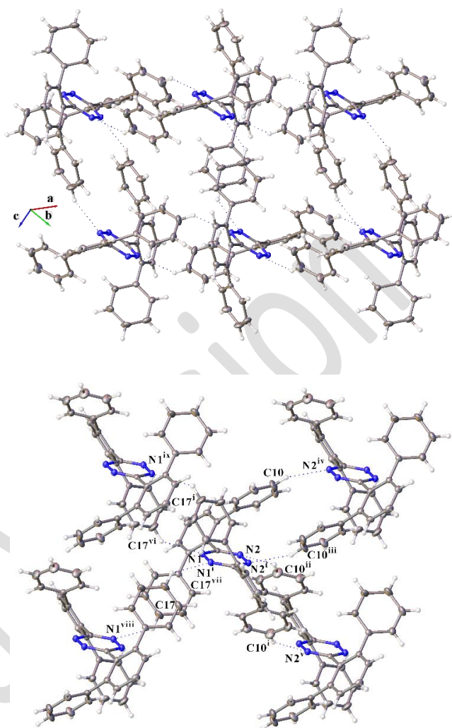
Fig. 6 View of the individual packing of conformers A' for 3 (top), and detail of intermolecular C–H...N hydrogen bonding network around a central molecule (bottom). Sym. Op.: (i) 1-x, y, 1.5-z , weak interactions C10–N2 : (ii) x, 2-y, -1/2+z , (iii) 1-x, 2-y, 2-z , (iv) x, 2-y, 1/2+z , (v) 1-x, 2-y, 1-z , weak interactions C17–N1 : (vi) x, -y, 1/2+z , (vii) 1-x, 1-y, 1-z , (viii) x, 1-y, -1/2+z , (ix) 1-x, 1-y, 2-z .
