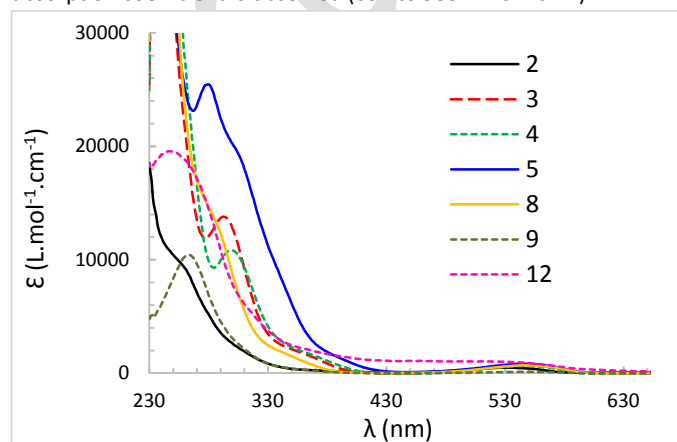
Fig. 15 Molar absorption coefficient of compounds of tetrazines 2 , 5 , 8 , 9 and 12 in dichloromethane at about 8.0 - 9.0 \cdot 10^{-5} M.
