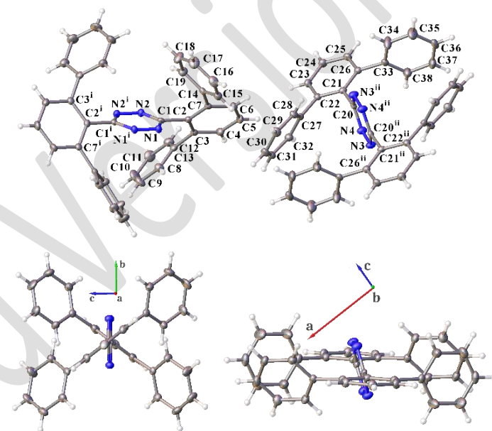
Fig. 4 Molecular structures of 3 showing 50% probability ellipsoids ( A' left, and B' right). Sym. Op.: (i) 1–x, y, 1.5–z, (ii) 0.5–x, 0.5–y, 1–z. Ct1 = C2–C3–C4–C5–C6–C7, Ct2 = C1–N1–N1 i –N2 i –N2–C1, Ct3 = C21–C22–C23–C24–C25–C26 and Ct4 = C20–N4–N3–C20 ii –N4 ii –N3 ii . Selected angles and torsions (deg.): A' : C3–C2–C1–N1 = 126.2(2); C3–C2–C1–N2 = –54.0(3), C7–C2–C1–N1 = –52.5(3); C7–C2–C1–N2 = 127.3(2); B' : C22–C21–C20–N3 ii = –103.7(2); C22–C21–C20–N4 = –73.8(2); C26–C21–C20–N3 ii = 78.2(2); C26–C21–C20–N4 = –104.4(2); intramolecular dihedral angles between Ct1 and Ct2 planes ( A' ): 52.53(5) and between Ct3 and Ct4 planes ( B' ): 75.60(6).
