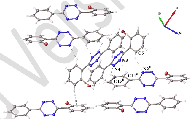
Fig. 2 Molecular structure and packing of 1-Br (ORTEP with 50% probability ellipsoids). Ct1 = C1(Br)-C2-C3-C4-C5-C6, Ct2 = C7-N1-N2-N3-N4-C8 and Ct3 = C9-C10-C11-C12-C13-C14. Hydrogen atoms have been omitted for clarity. Sym. Op. (i): 1-x, 1-y, 1-z, (ii) x, 0.5-y, 0.5+z. Selected bond length (Å), angles and torsions (deg.): intermolecular Ct1-Ct3i = 3.8547(13); intermolecular Ct2-Ct2i = 4.1285(11); C1-C6-C7-N1 = 39.5(3); C1-C6-C7-N3 = -144.5(2); C5-C6-C7-N1 = -141.2(2); C5-C6-C7-N3 = 34.8(3); C10-C9-C8-N2 = 158.9(2); C10-C9-C8-N4 = -19.2(3); C14-C9-C8-N2 = -21.9(3); C14-C9-C8-N4 = 160.1(2); Intramolecular dihedral angles between Ct1 and Ct2 planes 37.06(7), and between Ct2 and Ct3 planes 21.11(7).
