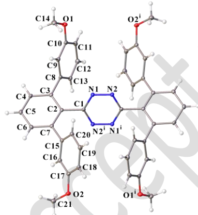
Fig. 12 Molecular structure of 10 (ORTEP with 50% probability). Ct1 = C2–C3–C4–C5–C6–C7, Ct2 = C1–N1–N2–C1'–N1'–N2'. Selected angles and torsions (deg.): C3–C2–C1–N1 = 60.89(15) ; C3–C2–C1–N2' = -118.51(12) ; C7–C2–C1–N1 = -120.70(12) ; C7–C2–C1–N2' = 59.91(14) ; intramolecular dihedral angles between Ct1 and Ct2 planes: 59.93(4) .
