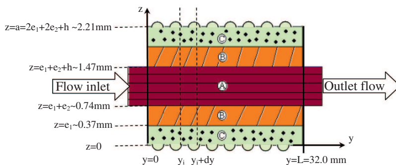
Fig. 10. Schematic geometry of the axial section of the plug flow filter press reactor used to perform simulations. Area A: Convection flow between both functionalized plates (section and volume of the flowing channel are respectively: 3.2 \text{ cm} \times 0.074 \text{ cm} = 0.237 \text{ cm}^2 and 3.2 \text{ cm} \times 0.074 \text{ cm} \times 3.2 \text{ cm} (or variable) = 0.757 \text{ cm}^3 ). Area B: Top layer of the immobilization matrix coating the enzymatic layer. Area C: Enzymatic layer.
