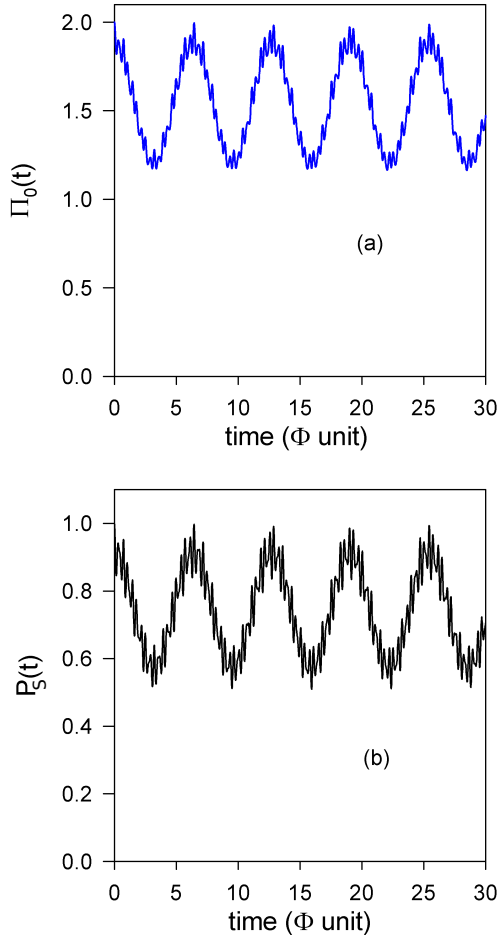
FIG. 7: Time evolution of (a) the exciton density and (b) the survival probability for A = 10.0 and N = 9 .
