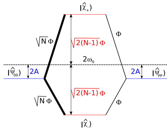
FIG. 3: Energy diagram of the 4-level system in which the two-exciton dynamics is confined.
