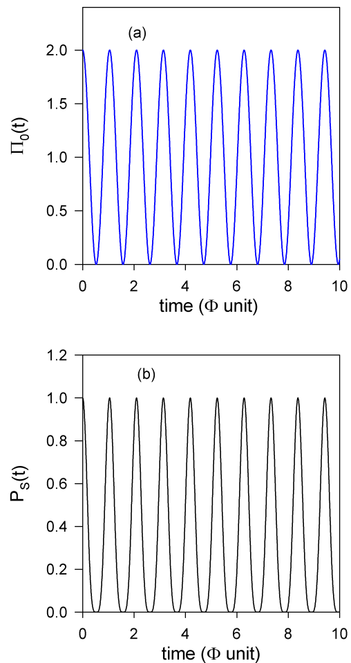
FIG. 4: Time evolution of (a) the exciton density and (b) the survival probability for A = 0 and N = 9 .
