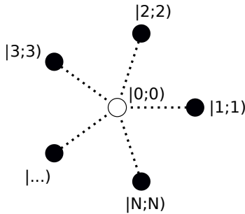
FIG. 11: Effective Hamiltonian that govern the pair states dynamics in the strong A limit. Full circles stand for the renormalized self-energy \tilde{\epsilon}_{pp} of the peripheral pair states |\ell; \ell\rangle whereas the open circle defines the renormalized self-energy \tilde{\epsilon}_{00} of the localized pair states |0; 0\rangle . Dashed lines represent the effective coupling J = -\Phi^2/A between the pair state localized on the core and the peripheral pair states (see the text).
