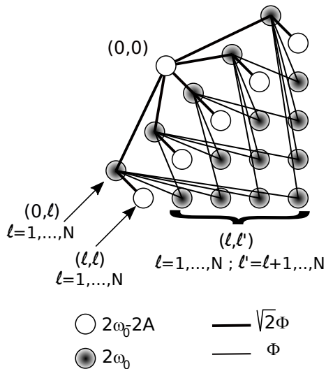
FIG. 2: Equivalence between the two-exciton Schrodinger equation and the dynamics of a single fictitious particle moving quantum mechanically on a complex network (see the text).
