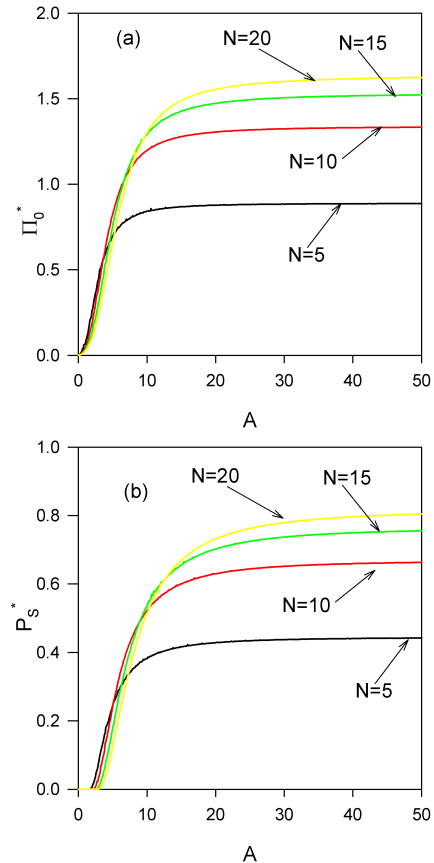
FIG. 8: A dependence of the minimum value of (a) the exciton density and (b) the survival probability over the timescale 100\Phi^{-1} and for different N values.
