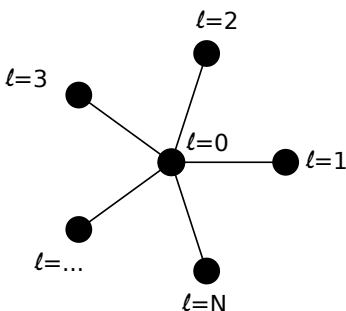
FIG. 1: The star graph.
