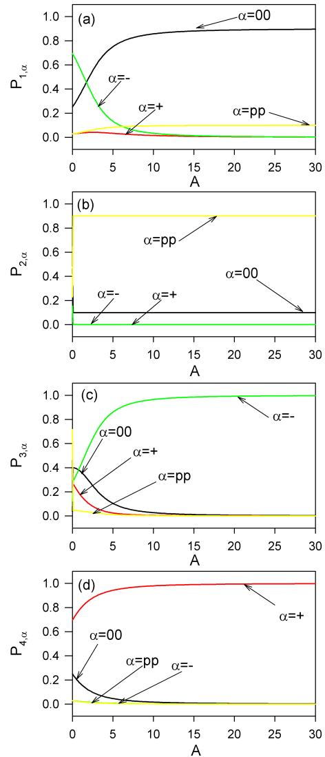
FIG. 10: A dependence of the two-exciton eigenstates in the four-dimensional active subspace for N = 9 .
