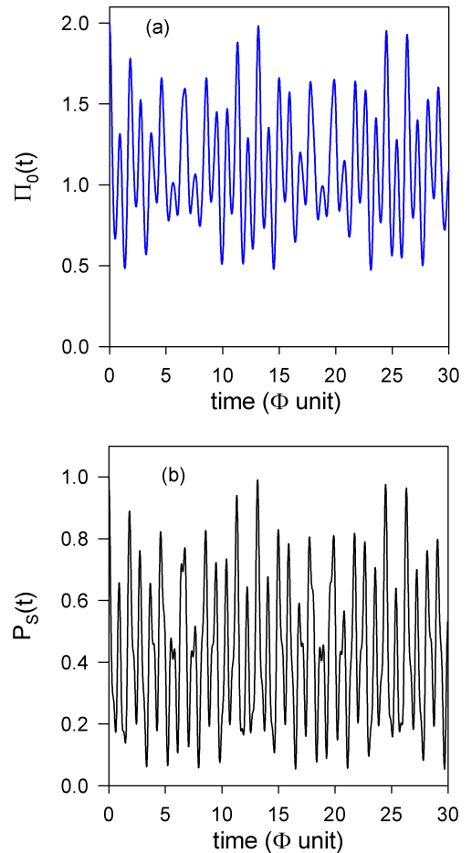
FIG. 6: Time evolution of (a) the exciton density and (b) the survival probability for A = 3.0 and N = 9 .
