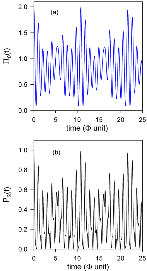
FIG. 5: Time evolution of (a) the exciton density and (b) the survival probability for A = 1.0 and N = 9 .
