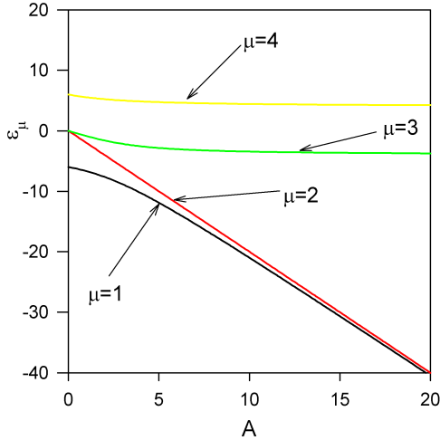
FIG. 9: A dependence of the two-exciton eigenenergies in the four-dimensional active subspace for N = 9 .
