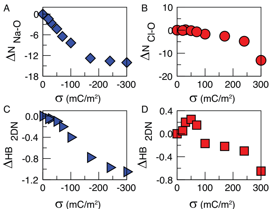
Fig. 5. Theoretical scores used to calculate the spectra shown in Fig. 2 D–F. (A) Differences in the total Na–O coordination numbers with respect to negative surface charging. (B) Differences in the total Cl–O coordination numbers with respect to positive surface charging. (C) Average number of HBs per molecule formed between water molecules in the topmost interfacial layer and oriented parallel to the surface for negative surface charging. (D) Average number of HBs per molecule formed between water molecules in the topmost interfacial layer and oriented parallel to the surface for negative surface charging.
