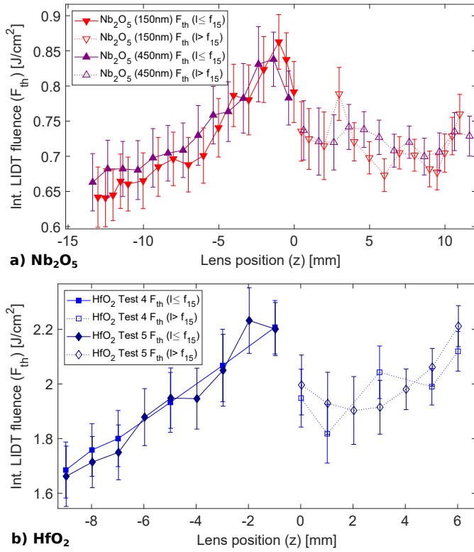
Fig. 7. Intrinsic LIDT fluence results for a) \text{Nb}_2\text{O}_5 and b) \text{HfO}_2 . The results are the same as in Fig. 6, but here they are plotted as a function of z lens position.
