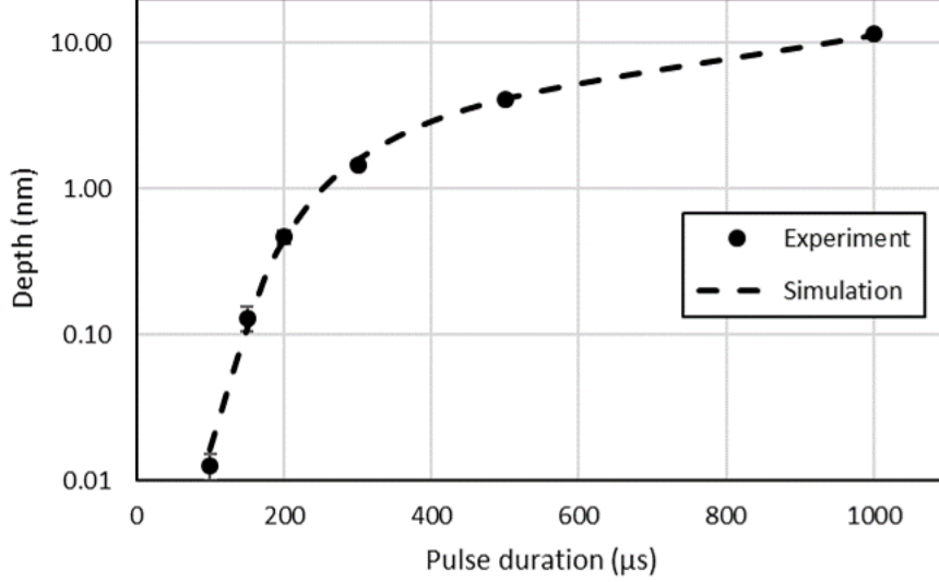
FIG. 7. Evolution of the depth of the craters with the pulse duration. The experimental data corresponds to a mean value on 30 sites, with the error bars given as plus/minus the standard deviation. The dashed line corresponds to the numerical simulations.
