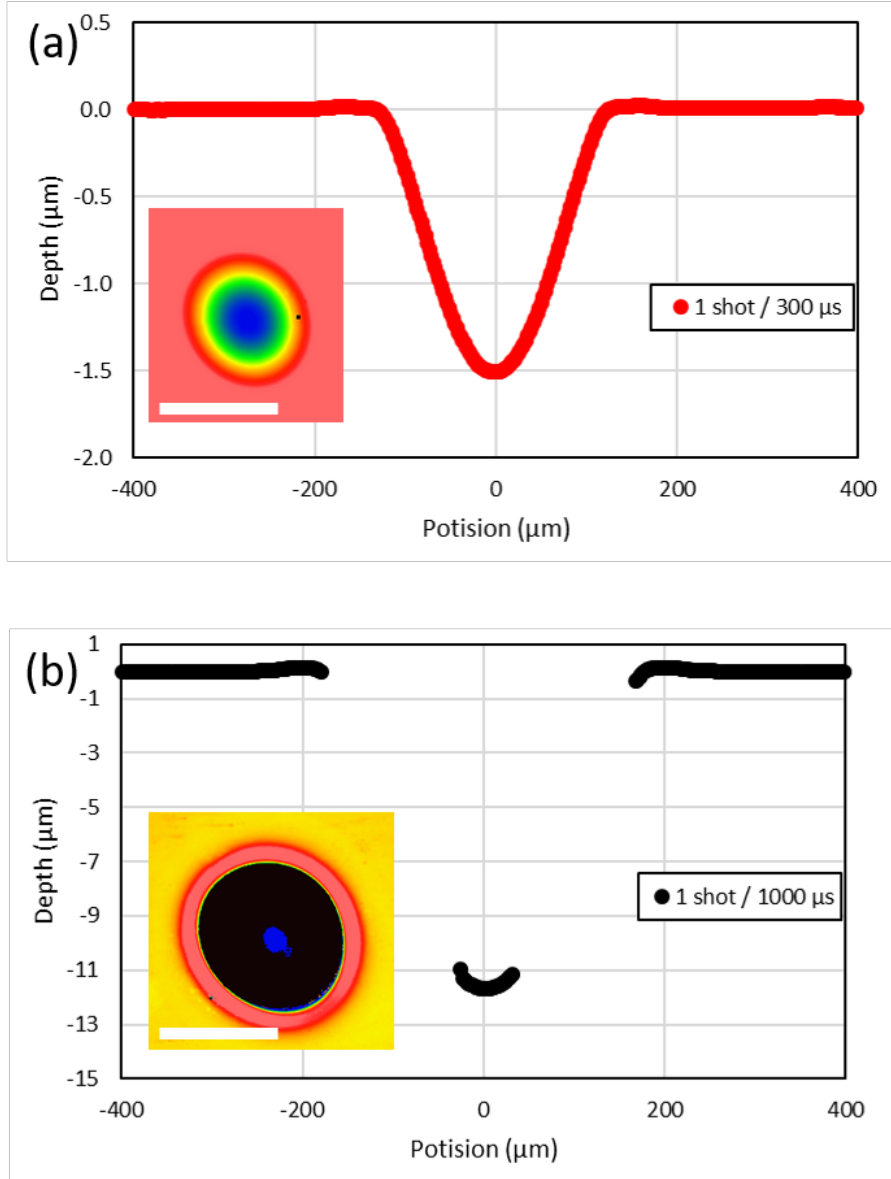
FIG. 6. Surface profiles measured with optical profilometer. The inserted images show the surface topography with a scale bar of 200 \mu\text{m} . Irradiation conditions (a) 300 \mu\text{s} , 85W ; (b) 1000 \mu\text{s} , 85W.
