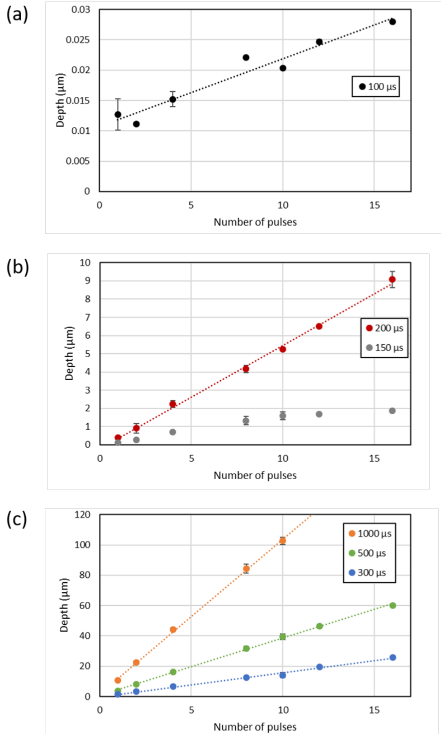
FIG. 8. Evolution of the depth of the craters with the number of pulses for different pulse durations. (a) Case of 100 \mu\text{s} pulses ; (b) 150 and 200 \mu\text{s} ; (c) 300, 500 and 1000 \mu\text{s} . The dashed line corresponds to a linear fit of the data (in the case of pulses of 150 \mu\text{s} the evolution was non linear).
