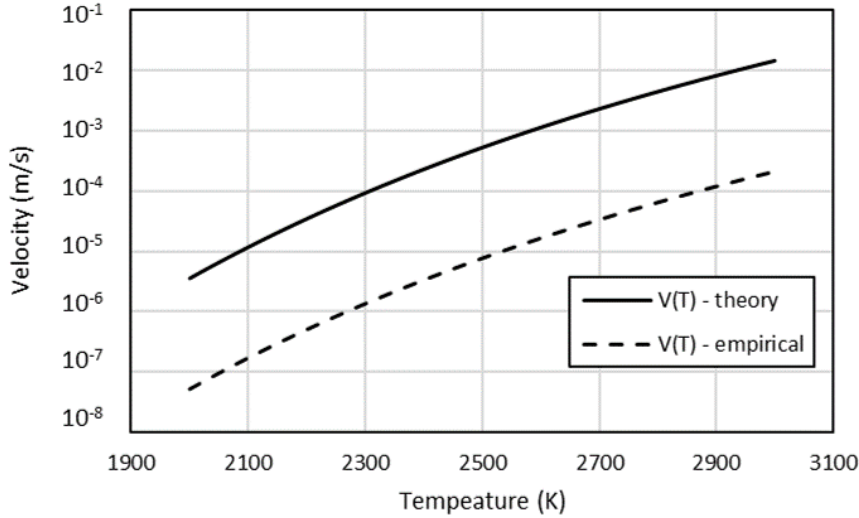
FIG. 4. Velocity of the evaporation front as a function of temperature. Plain line curve corresponds to the theoretical velocity calculated from the kinetic theory of gas. Dash line curve corresponds to the velocity determined from experiments (effective velocity) with the application of \beta coefficient.
