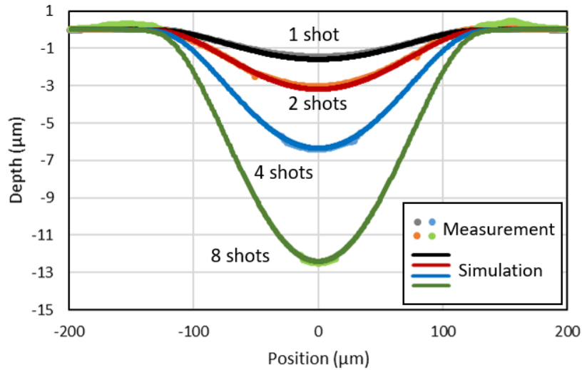
FIG. 10. Measured crater profiles and comparison to simulations. Case of successive irradiations on the same site.
