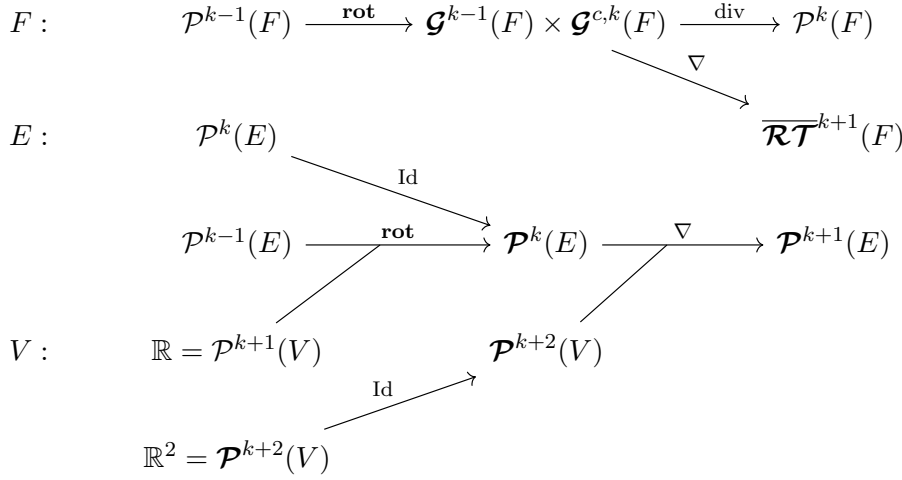
Figure 1: Usage of the local degrees of freedom for the discrete differential operators.
