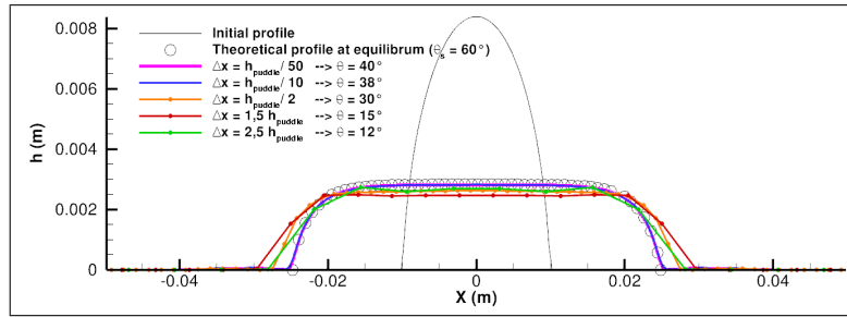
FIGURE 8 – Equilibrium profiles with \theta_s = 60^\circ for various values of mesh size \Delta x . The value h_{puddle} ( = 2 l_c \sin(\theta_s/2) ) corresponds to the liquid film thickness far from the triple line. For each case, the value of the calculated apparent contact angle \theta is given in the legende.
