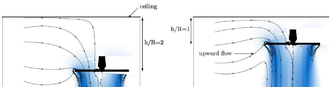
Figure 6. Streamlines and iso-lines of radial fluctuating velocities superimposed to contours of velocity magnitude. Flowfields obtained for the h/R=2 (left) and h/R=1 (right) ICE configurations.
