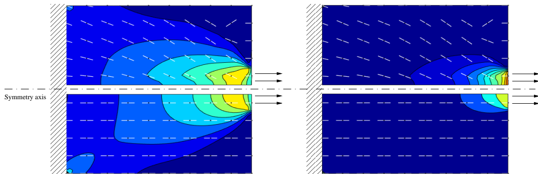
Figure 2: 2D body under boundary traction. White lines represent material orientation before (bottom) and after (top) remodeling. Left: strain energy density (color map, arbitrary units). Right: Von Mises stress (color map, arbitrary units).
