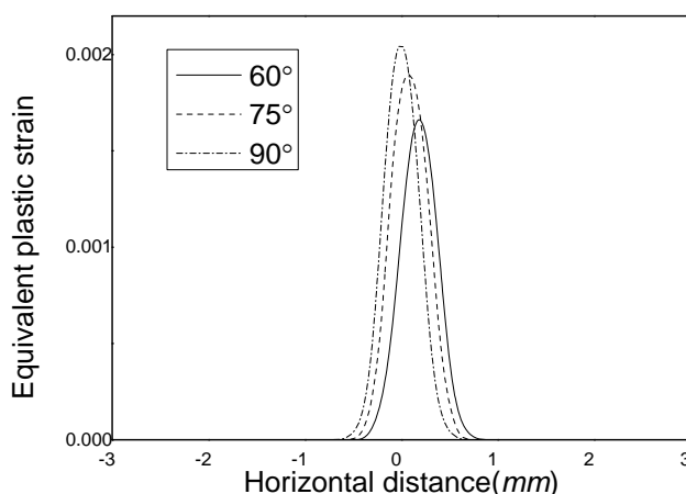
Fig. 6. Plastic strain induced by impacts following different impact angles.
