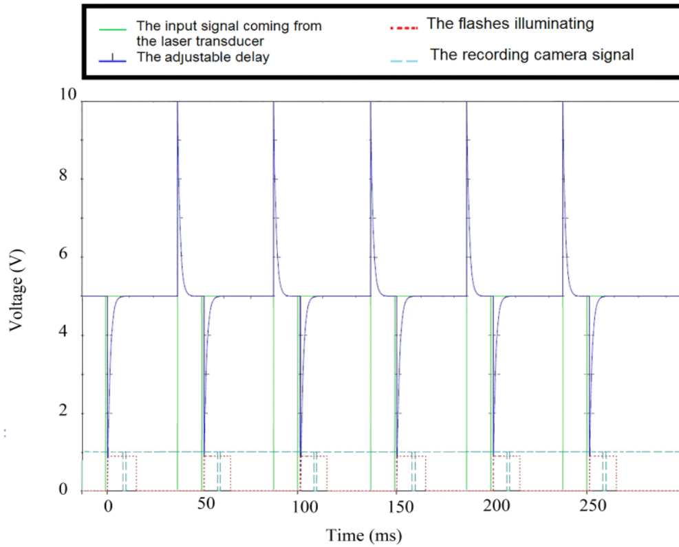
Figure 4: Signal chart.
