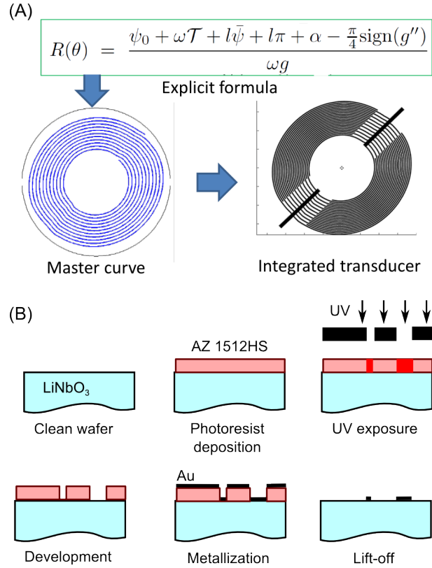
Figure 2: Design and fabrication of the acoustic vortex integrated transducers. (A) Design: Eq. (6) is evaluated numerically, resulting in a master curve. This master curve is converted to photomask using a home-made Python algorithm (available in the supplemental material of [12]). (B) Fabrication: A clean X-cut of lithium niobate is coated by the AZ 1512HS positive photoresist. Using the photomask designed above, a section of the resin is insulated and removed using a developer. 50 nm of chromium and 200 nm of gold are then deposited on the wafer by e-beam evaporation. Finally, the lift-off step removes the excess resin and metal.
