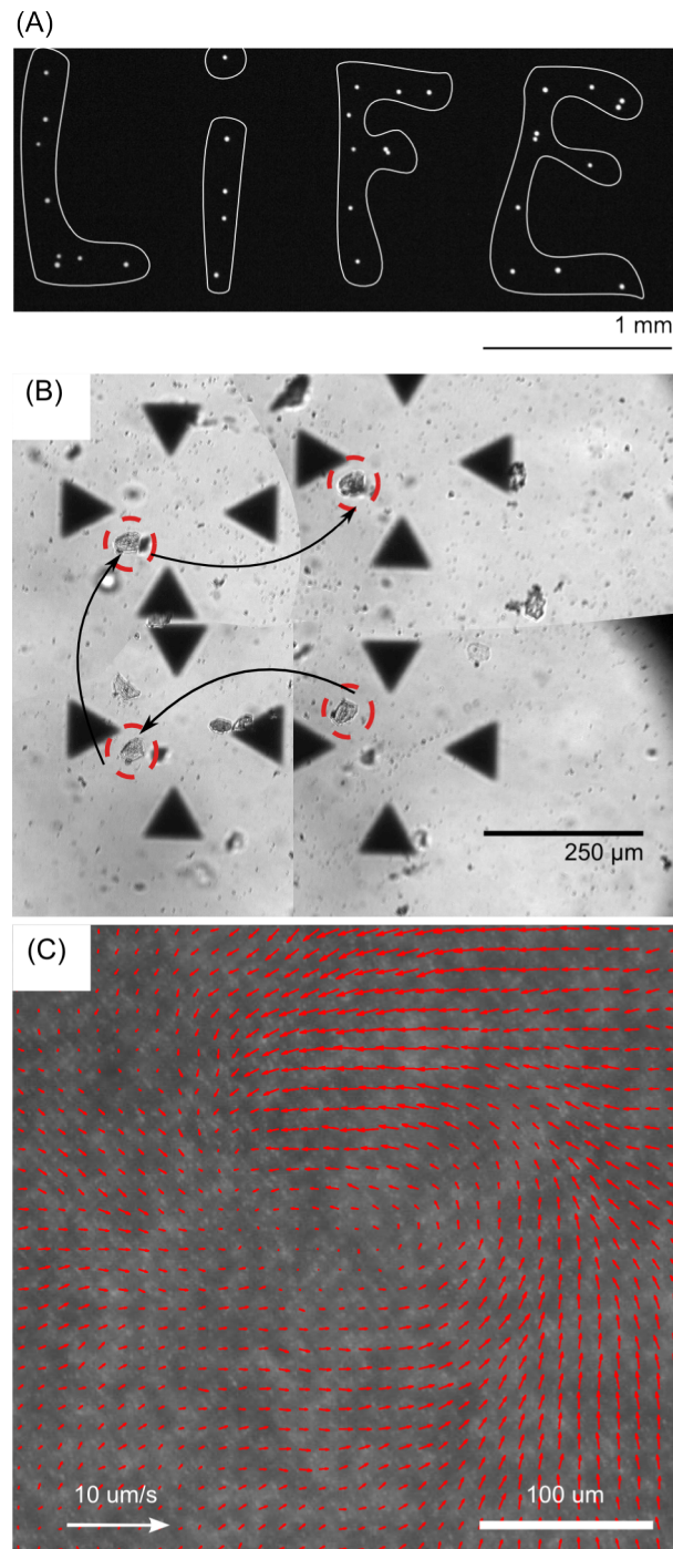
Figure 4: Manipulation of fluids and particles with an integrated acoustical tweezer. (A) Patterning: Final arrangement of 33 PS beads (diameter 30 \mu\text{m} ) initially randomly dispersed. (B) Cell manipulation: a buccal epithelium cell is trapped by the acoustic vortex and displaced relatively to the sample. (C) Vorticity generation: PIV snapshot of the swirling flow motion generated by acoustic streaming around the vortex core.
