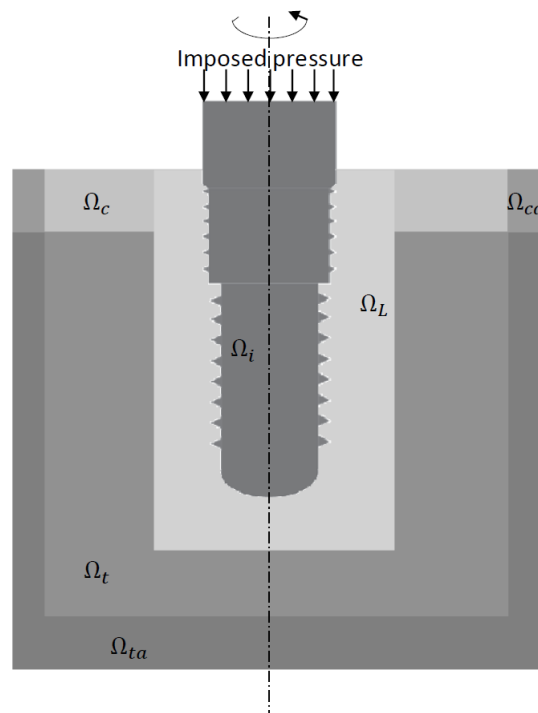
Figure 1: Cross-section view of the 3-D axisymmetric geometrical configuration used in the numerical simulations. The domains are denoted with a subscript corresponding to the variable material ( \Omega_L ), the trabecular bone ( \Omega_t ), the cortical bone ( \Omega_c ), the implant ( \Omega_i ), and the absorbing layers associated to trabecular and cortical bone ( \Omega_{ta} and \Omega_{ca} , respectively).
