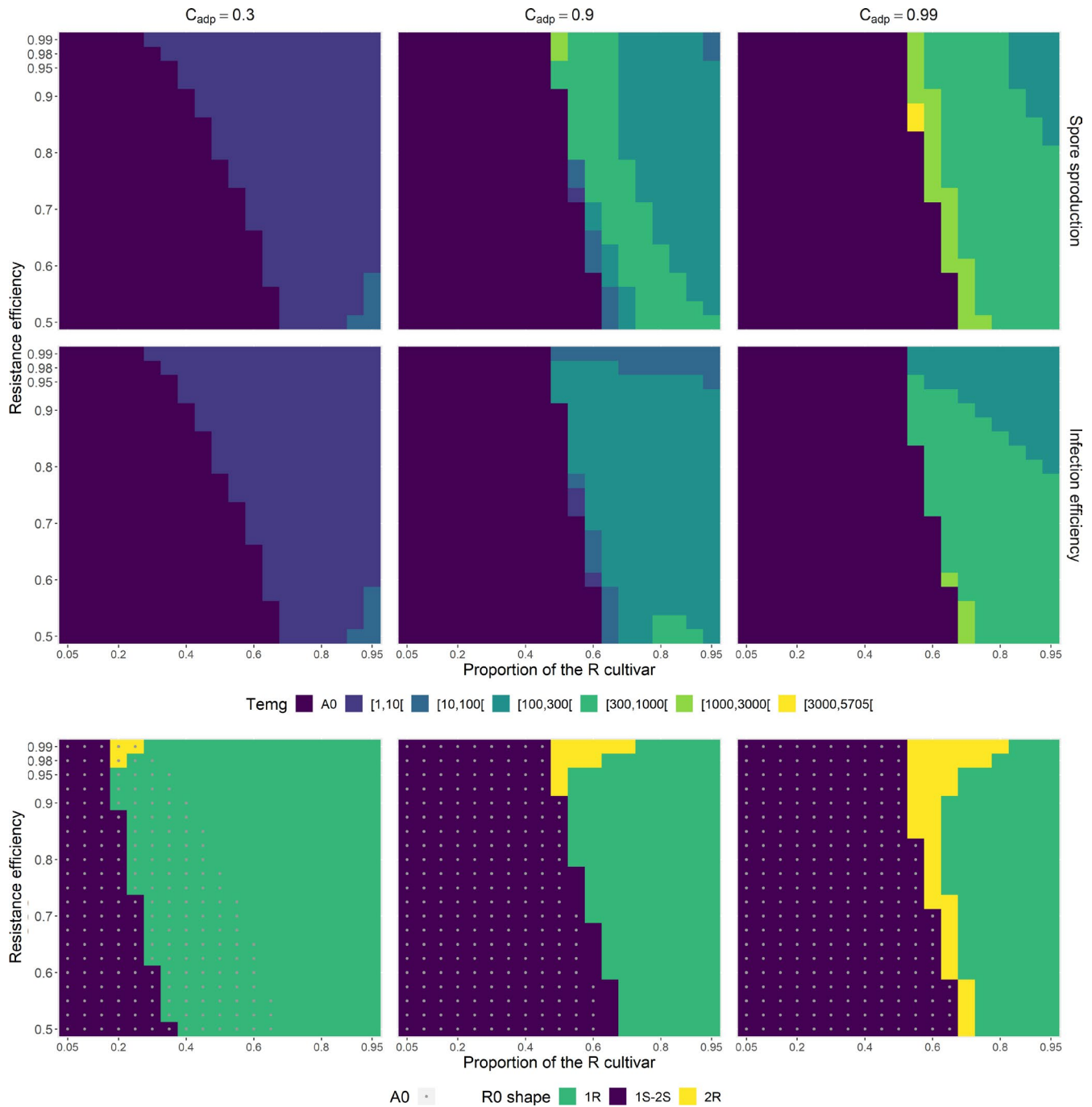
FIGURE 4 Time to emergence of the evolutionary attractor. The time to emergence T_{emg} is the time at which the proportion of the evolutionary attractor (the closest to the optimal phenotype on the R cultivar) becomes \geq 5\% in the pool of spores in the air. Line 1. The resistance affects only total spore production (SP scenario). T_{emg} is characterized as a function of the proportion of the R cultivar at planting (x-axis) and of the relative effectiveness of the resistant cultivar (y-axis) for three costs of adaptation (columns). Level A0 indicates situations in which the criteria for emergence are met right from the initial conditions. Line 2. An in line 1 when the resistance affects only infection efficiency (IE scenario). Line 3. Shape of the \mathcal{R}_0 function. Three shapes are classified: (i) "1S-2S" when the evolutionary attractor \mu^* is closer to \mu_S than to \mu_R (i.e., \mu^* < 0 ), (ii) "1R" when \mu^* is closer to \mu_R and \mathcal{R}_0 is unimodal, and (iii) "2R" when \mu^* is closer to \mu_R and \mathcal{R}_0 is bimodal. Point A0 indicates situations in which the criteria for emergence are met right from the initial conditions. For all panels, all the other parameters are set to their reference values (Table 2)
