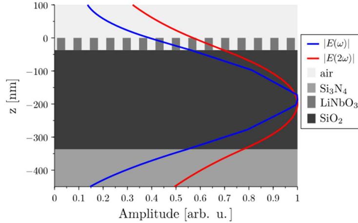
Figure 7: Normalized modulus of the electric field at x=0 with respect to z , at the pump and harmonic frequencies.
