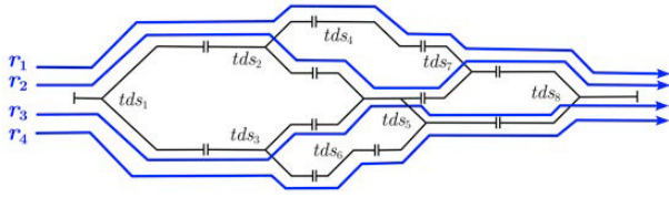
Fig. 5. Example of tds sequences to illustrate group constraints
