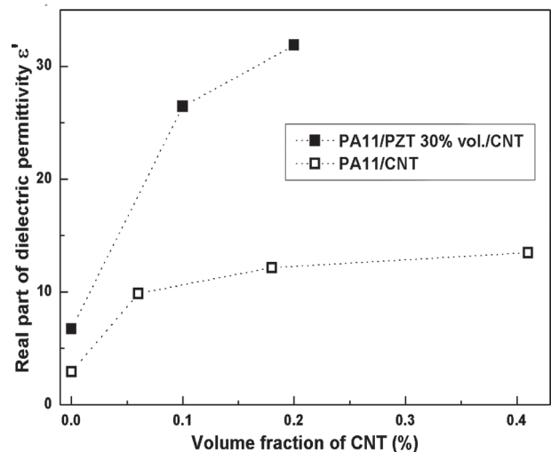
Fig. 5. Real part of the dielectric permittivity \epsilon' of PA11/PZT 30 vol%/CNT and of PA11/CNT composites as a function of CNT volume fraction.
