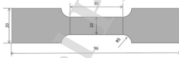
Figure 1: Uniaxial tensile test specimen according to the ISO 80/20 norm
