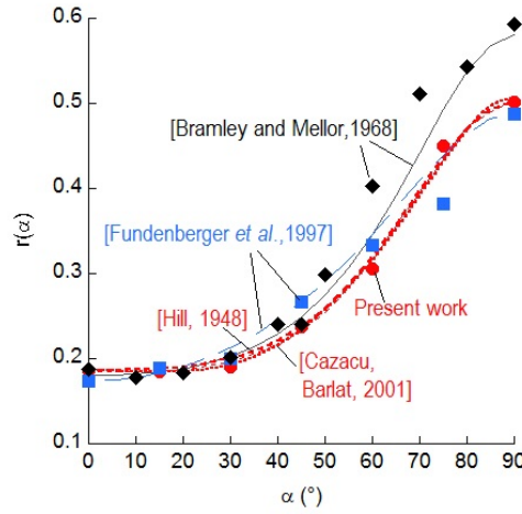
Figure 14: r-value prediction using (\sigma_0^0, r_0, r_{45}, r_{90}) for the identification of F , G , H and N or the set of all experimental data (present work). The results obtained using the Cazacu-Barlat criterion [39] are also indicated. For comparison purpose, data from Bramley and Mellor [12] and Fundenberger et al [27] are provided.
