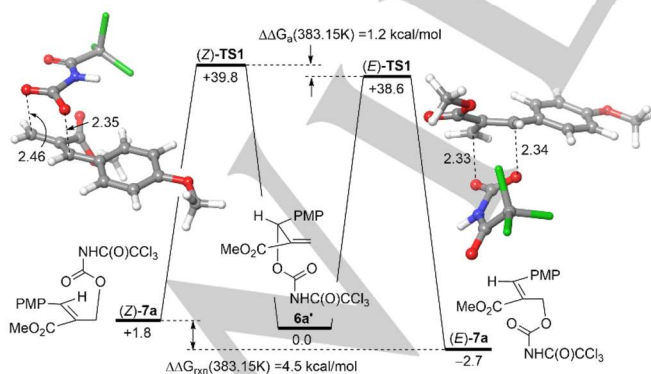
Figure 2. Reaction profile of the dioxo-[3,3] sigmatropic shift of carbamoyl intermediate 6a' to both ( E ) and ( Z ) isomers of 7a , computed at the M06-2X(PCM,toluene)/6-31+G* level of theory. Relative free energies, in kcal/mol, have been computed at 383.15 K. Bond distances are given in Å.
