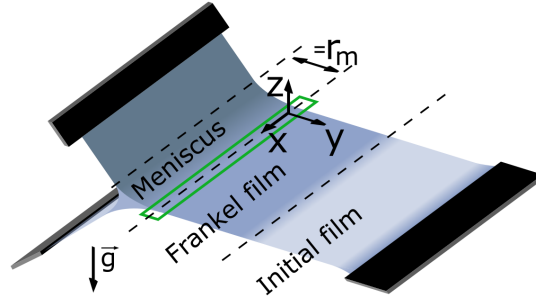
FIG. 2. Sketch of the experimental setup. Three films extend between a free meniscus and mobile frames, and the film of interest is the horizontal one in the xy -plane. To produce a reproducible initial condition, a piece of film of controlled thickness (of the order of one micron), denoted as the Frankel film , is extracted from the free meniscus by stretching the horizontal film. The green rectangle represents the area of interest pictured in Figure 4. The meniscus on the mobile frame (on the right) behaves similarly but is not studied.
