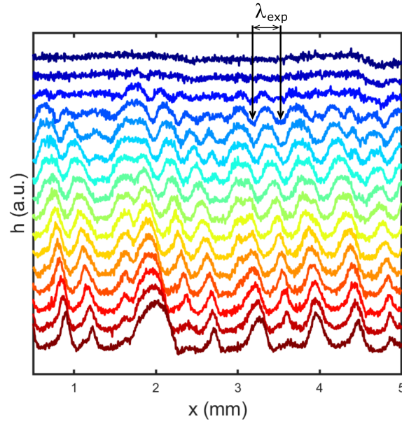
FIG. 5. Intensity profiles along the line y = y_p (shown in Fig. 4) recorded every 10 ms, from t = 0 (top, dark blue) to t = 150 ms (bottom, dark red). A arbitrary offset is added for the sake of visibility.
