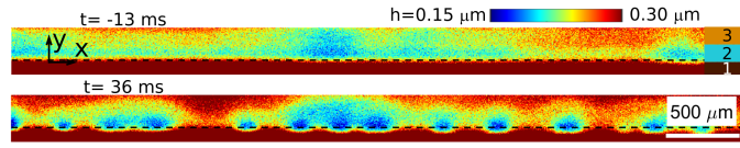
FIG. 4. Film thickness field obtained from the fluorescence intensity before (top, t = -13 ms) and after (bottom, t = 36 ms) the instability onset ( h is the half-thickness). The bars on the right of the top image indicate the meniscus (region 1, thickness not resolved), the pinched region, of width w_p (region 2), and the Frankel's film, of thickness 2h_\infty (region 3). The region pictured correspond to the rectangle shown in Fig. 2, and the dashed line is the position y_p where the profiles of Fig. 5 are measured.
