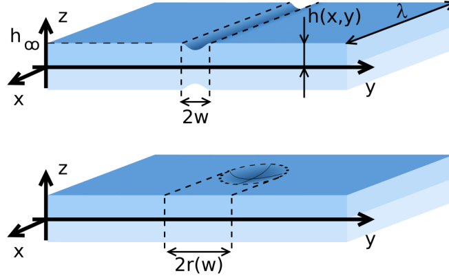
FIG. 8. The Gaussian profile in the domain \mathcal{P}_\lambda (top) and its reorganized axisymmetric shape (bottom).
