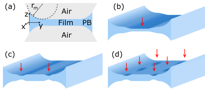
FIG. 1. (a) Sketch of the studied configuration: a flat film of surfactant solution separates two volumes of air (bubbles), and is delimited by two Plateau borders (PB) of uniform radius of curvature r_m . Under the assumption of a thickness uniform along the x direction, different cases are known for the drainage depending on the boundary condition at the interfaces: the thinnest part of the film can be located in the center (b) or at the edges of the film (c). In the experiments and in the present modeling, the thickness profile is close to case (c) at short time. However, it does not remain uniform along the x direction at long time, and destabilizes into a periodic pattern (d).
