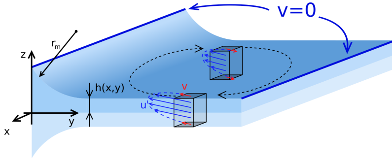
FIG. 7. Notations used in the text and schematic of the most general flow pattern, associated with the equations (3- 5).
