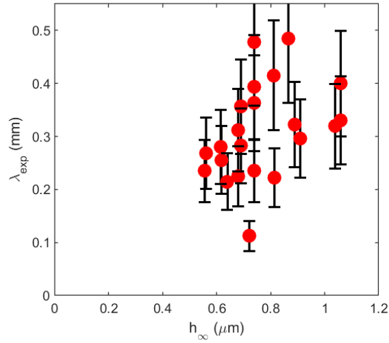
FIG. 6. Measured wavelengths as a function of the thickness of the flat Frankel film.
