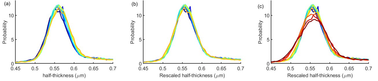
FIG. 10. (a) Probability distribution function of the film half-thickness h in the vicinity of the pinched region, recorded every 5 ms from t = -10 ms (dark blue) to t = 25 ms (orange). (b) Same data, after a global rescaling, taking into account a residual compression of the film. (c) Same data as in b , with three additional times 30, 35 and 40 ms.
