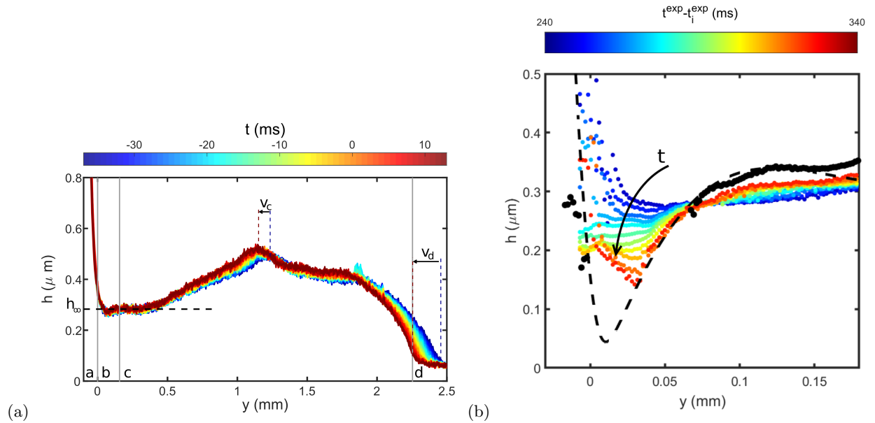
FIG. 3. (a) Film profile ( h is the half thickness) from fluorescence measurement calibrated through the spectral camera, close to the destabilization time at t = 0 (in this example t_i = -450 ms). Areas a, b, c and d respectively correspond to the meniscus, the pinched region, the Frankel film, and the initial thin film. Two characteristic material points can be followed during this time range and move at the velocities v_c = 1.6 mm/s, and v_d = 4.0 mm/s indicated in the figure, showing the film compression. (b) Zoom on the 1D film profiles obtained with the spectral camera for the same experiment, before the destabilization. The colored profiles are recorded from t = -210 ms (dark blue) to -110 ms (red) every 10 ms and the black one shows the measurable part of the profile at t = 0 ms.
