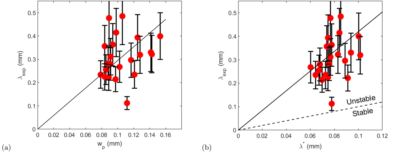
FIG. 11. Experimental wavelength \lambda_{exp} as a function of the pinched region width (a) and as a function of \lambda^* (b). The solid lines are guides for the eyes, of equation \lambda_{exp} = 2.95 w_p on the left and \lambda_{exp} = 4.2 \lambda^* on the right. The dashed line corresponds to \lambda_{exp} = \lambda^* .
