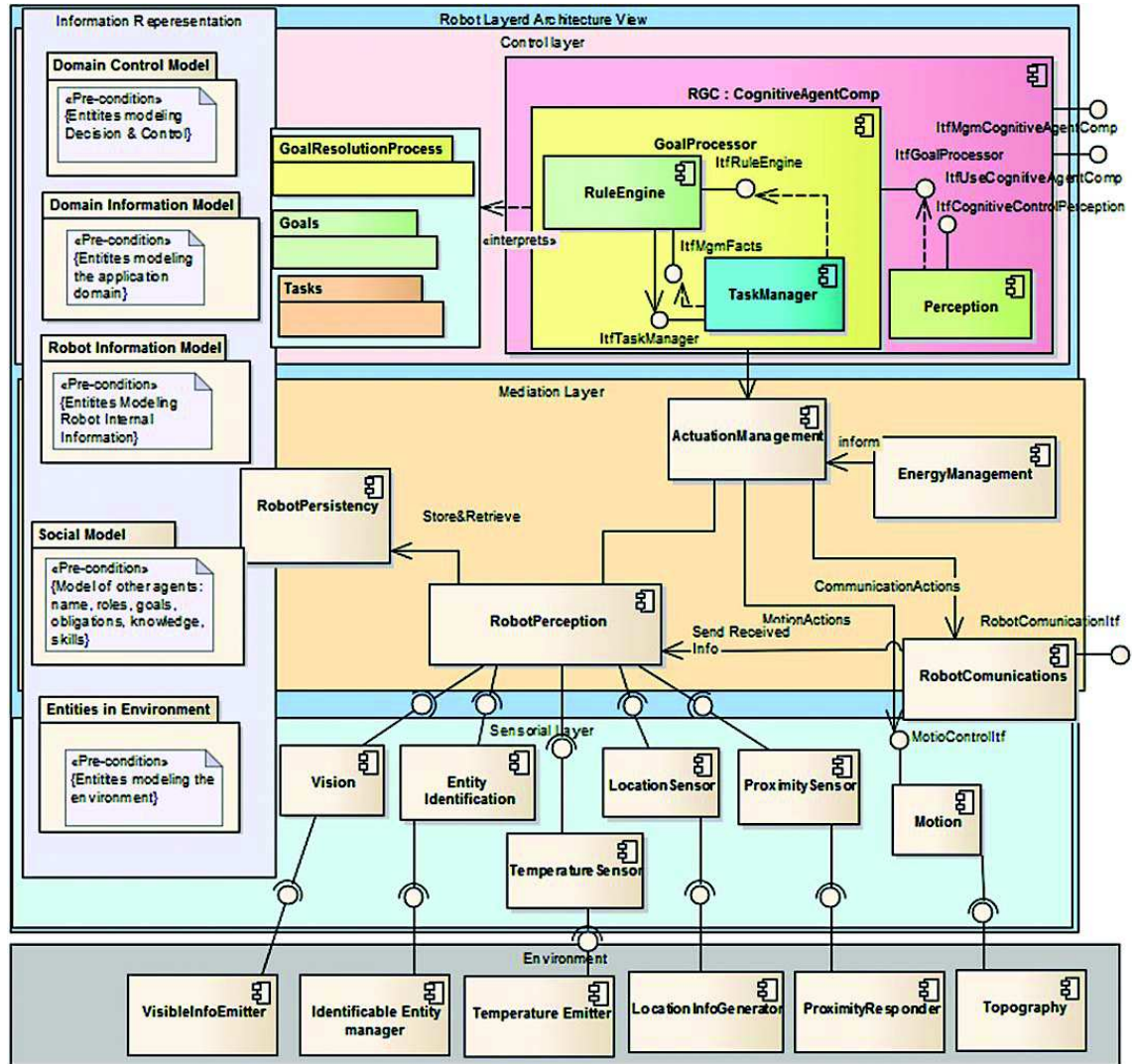
Fig. 1. The general multi-layered component-based architecture.
