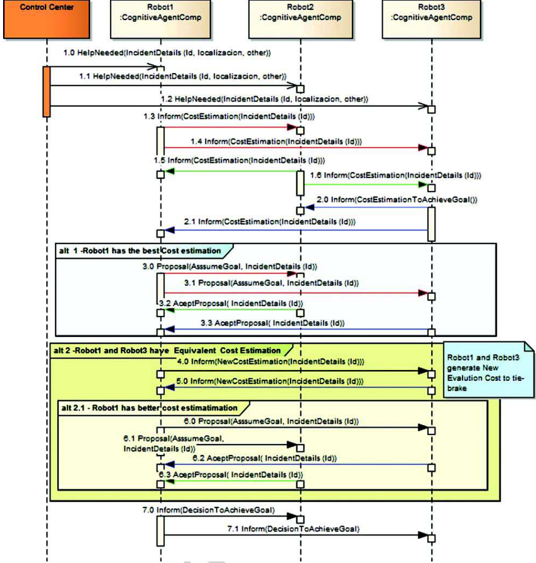
Fig. 2. The adaptive multi-agent system (AMAS) cooperation model.
