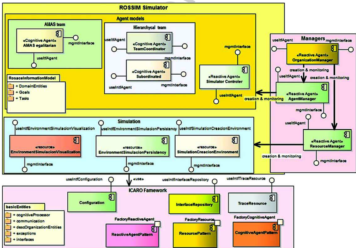
Fig. 4. Simulator architecture implemented with ICARO.
