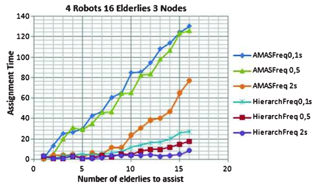
Fig. 6. AMAS versus hierarchical model.
