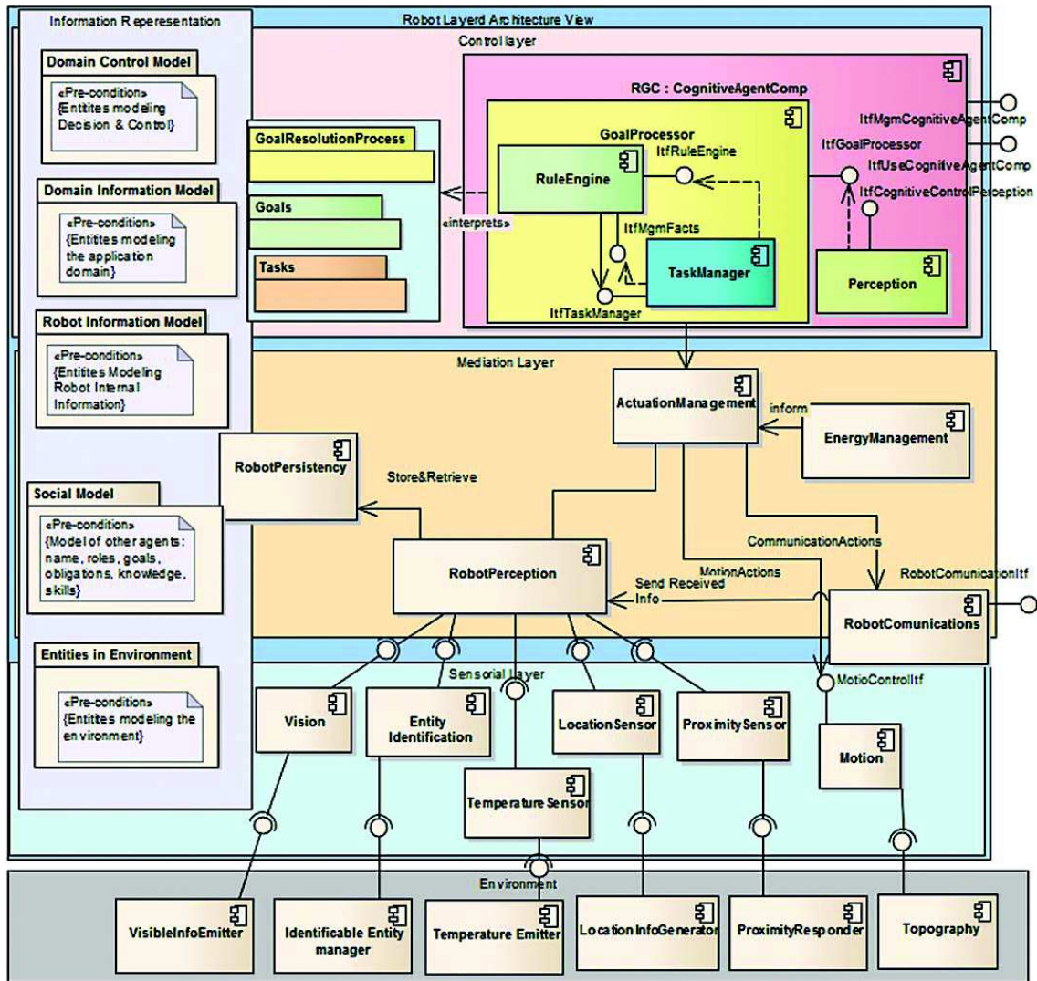
Fig. 1. The general multi-layered component-based architecture.
