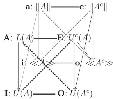
Figure 4. Cube of oppositions induced by rough approximations
