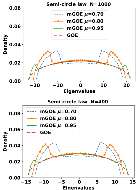
FIG. 1. Semicircle law of mixed GOE with different degree of mixing and non-mixing for N=400 and N=1000 over 100 draws, i.e., ensemble size.
