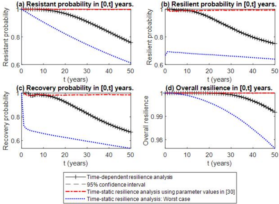
Fig. 11: Comparison to time-static resilience analysis.
