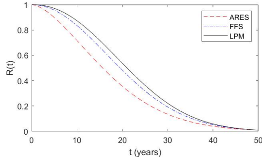
Fig. 10: Reliability of the three major safety barriers.
