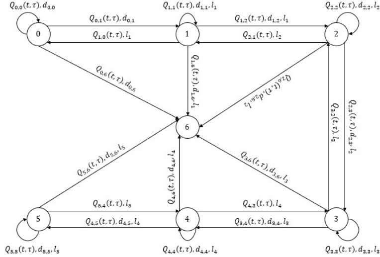
Fig. 6: State transition diagram of the NHSMRP.
