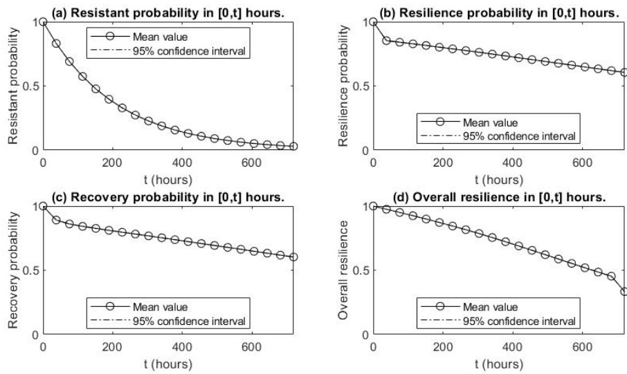
Fig. 13: Time-dependent resilience analysis for the computing system.
