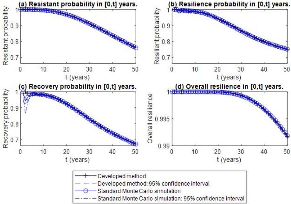
Fig. 9: Time-dependent resilience analysis (Sample size: 10^6 ).
