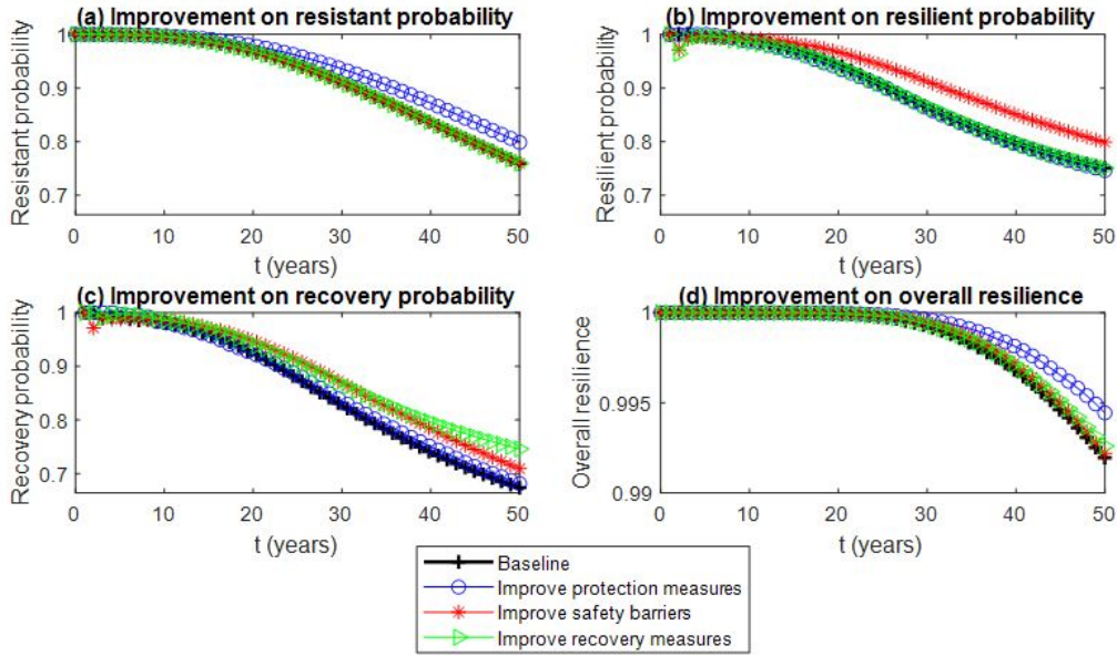
Fig. 12: Effectiveness of different improvement measures.
