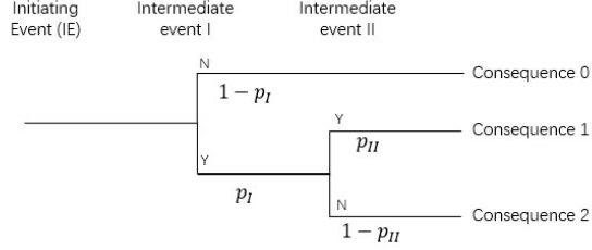
Fig. 4: An illustration of an event tree
