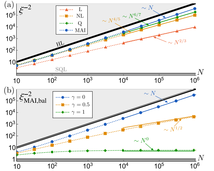
FIG. 1. Scaling laws for the quantum gain. (a) The quantum metrological gain \xi^{-2} optimized over the preparation time \chi t for linear (L), nonlinear (NL), quadratic (Q), and MAI measurement strategies as a function of N compared to the standard quantum limit (SQL) and the Heisenberg limit (HL). Solid lines represent the analytical scaling laws in the limit of large N including finite size corrections. The leading term is indicated in the plot. (b) Modification of the scaling laws for the MAI method in the presence of ballistic noise with fluctuations that scale with \gamma for \epsilon = 0.05 (see text).
