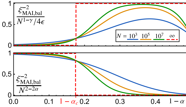
FIG. 2. Discontinuous scaling law in the presence of ballistic dephasing. Quantum metrological gain of the MAI method \xi_{\text{MAI,bal}}^{-2} with \tau = -t , \epsilon = 0.05 , \gamma = 0.65 as a function of \alpha : Larger values of 1 - \alpha correspond to longer preparation times as we set \chi t = \sigma N^{-\alpha} . The normalized quantum gain \xi_{\text{MAI,bal}}^{-2}/(N^{1-\gamma}/4\epsilon) (top) and \xi_{\text{MAI,bal}}^{-2}/N^{2-2\alpha} (bottom) illustrates how the scaling in the thermodynamic limit, Eqs. (7) and (8) for short and longer times, respectively, is approached as N increases. At \alpha_c (6) the transition becomes discontinuous in the thermodynamic limit.
