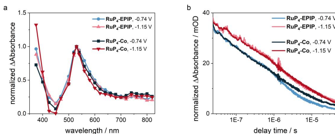
Figure 4. a) TA spectra of RuP 4 -EPIP- and RuP 4 -Co- sensitized NiO films at -0.74 V and -1.15 V vs Fc +0 applied potential at 100 ns time delay, normalized to signal at 530 nm. b) Kinetic traces at 530 nm of the same data, averaged from 520 to 540 nm and normalized at 30 ns to the signal of RuP 4 -Co at the respective potential.
