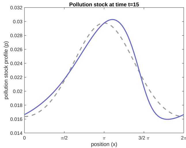
FIGURE 7. Comparison of the pollution spatial distributions, sections at t=15 , the dashed curve for the benchmark case with constant diffusion speed.
