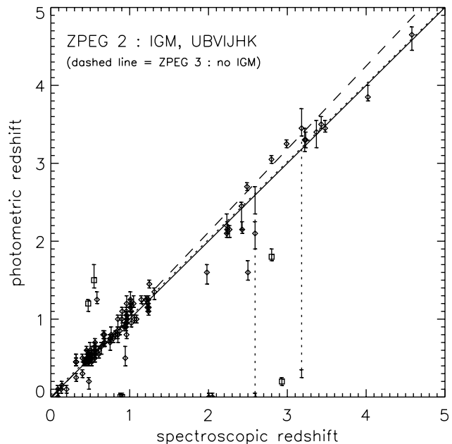
Fig. 5. Photometric redshift estimations like in Fig. 2 when our computations are free of any age constraint (model Z-PEG.2 ). The dotted diagonal line is the linear regression of points with |z_{Z-PEG} - z_{\text{spe}}| < 1 . The dashed line is the linear regression without the IGM absorption (model Z-PEG.3 ).
