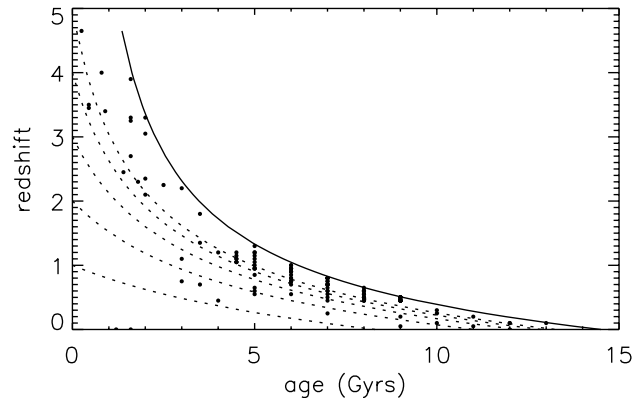
Fig. 8. Galaxies of the HDF-N sample in the redshift–age diagram, after Z-PEG fits. The dotted lines show the z -age relations for various z_{for} (iso- z_{for} lines) and the standard cosmology, previously defined. For example, the dotted line crossing the y -axis (age = 0) at z = 2 corresponds to z_{for} = 2 . The solid line shows the age of the universe at a given redshift (formally, this line is equivalent to z_{for} = \infty ). As a result, most galaxies form at z > 3 (we can also check this result in Fig. 9).
