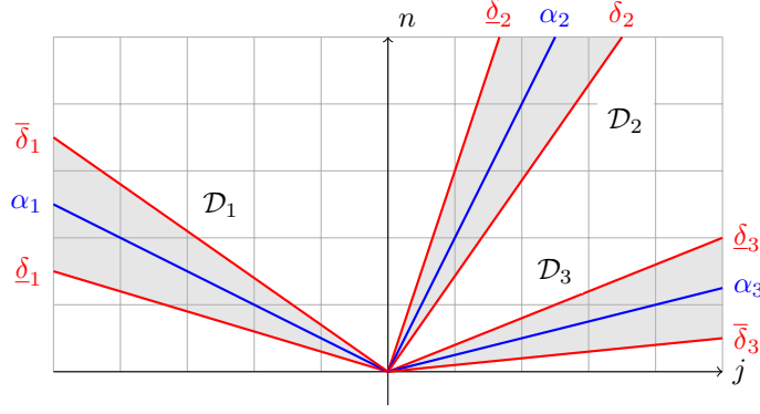
Figure 4: An illustration of the sectors \mathcal{D}_k . Here, we have \alpha_1 = -2 , \alpha_2 = 0.5 and \alpha_3 = 4 . The rays labeled \alpha_k (resp. \delta_k , \bar{\delta}_k ) correspond to the ray j = n\alpha_k (resp. j = n\delta_k , j = n\bar{\delta}_k ). We observe that, because \delta_k , \alpha_k and \bar{\delta}_k have the same sign, j and \alpha_k have the same sign for (n, j) \in \mathcal{D}_k . Also, the sectors \mathcal{D}_k do not intersect each other.
