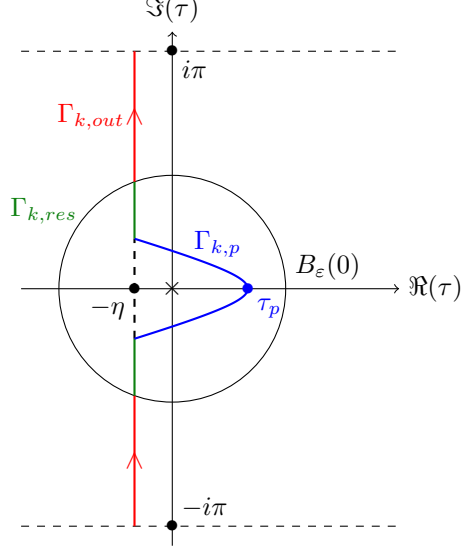
Figure 5: A representation of the path \Gamma_k for \tau_k = 0 . It is composed of \Gamma_{k,out} (in red), \Gamma_{k,res} (in green) and \Gamma_{k,p} (in blue). The section of \Gamma_k which lies inside the ball B_\varepsilon(\tau_k) (i.e. the reunion of \Gamma_{k,res} and \Gamma_{k,p} ) is notated \Gamma_{k,in} .
