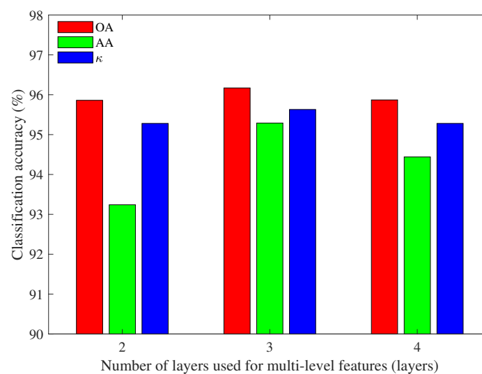
Figure 9. Classification accuracy of Indian Pines based on multi-level features with different numbers of encoded layers.
