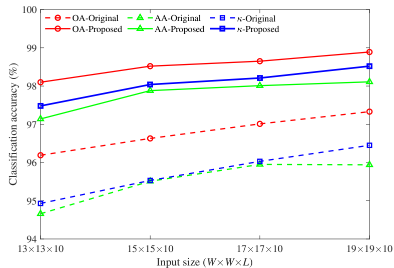
Figure 6. Classification accuracy of Pavia University under different input sizes.
