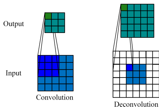
Figure 2. 2D convolution and 2D deconvolution.
