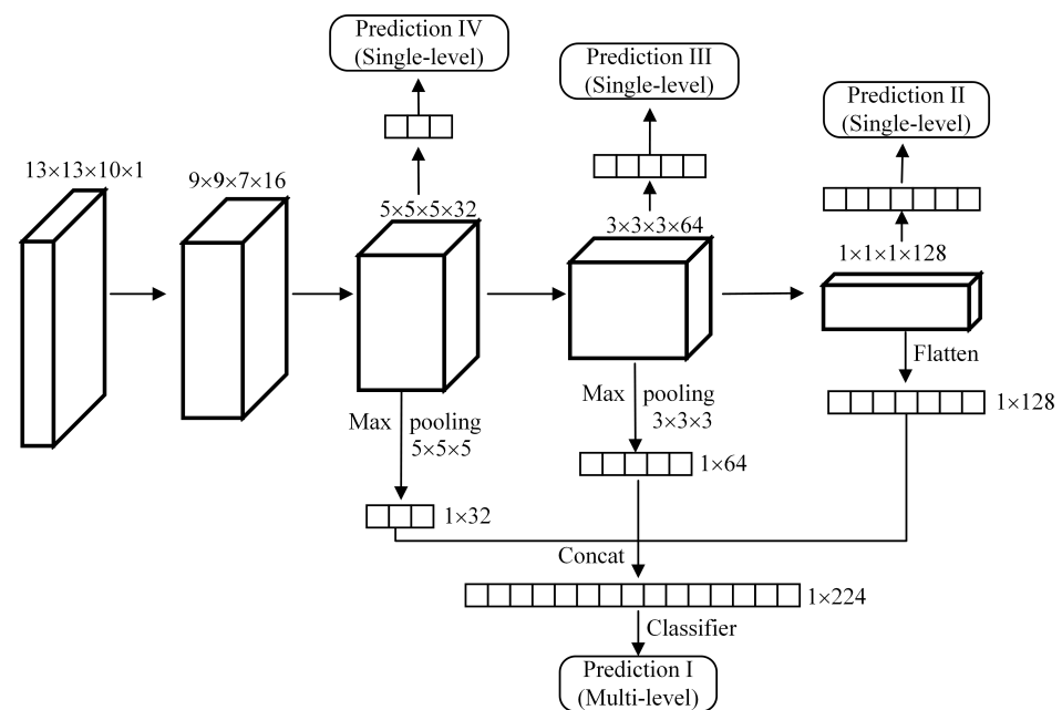
Figure 5. Different features from the encoder of 3D-CAE for classification.
