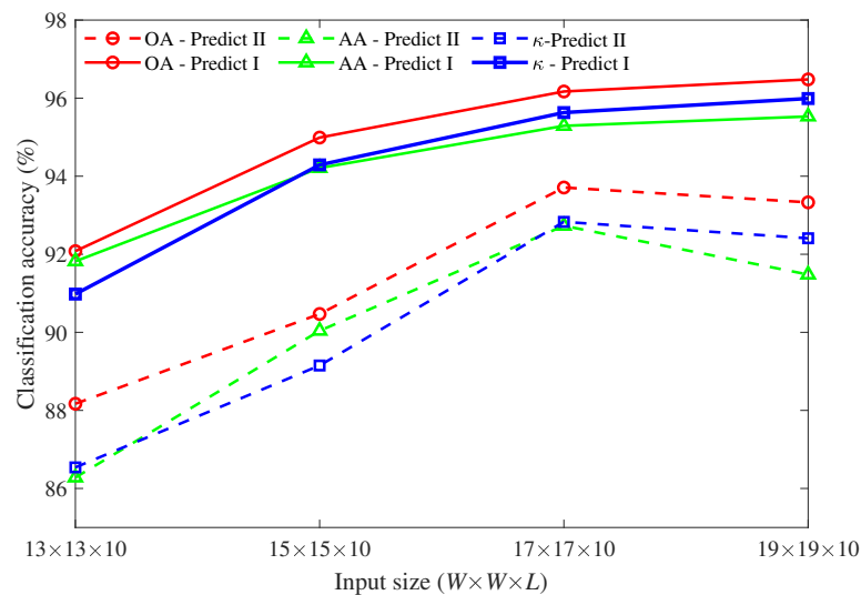
Figure 7. The classification accuracy of Indian Pines under different input sizes.
