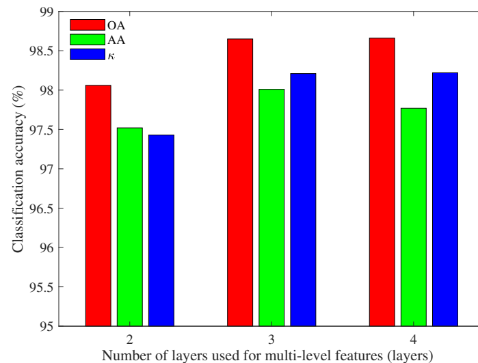
Figure 8. Classification accuracy of Pavia University based on multi-level features with different numbers of encoded layers.
