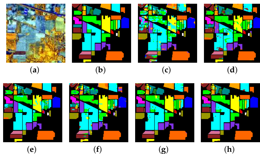
Figure 11. Indian Pines: (a) Composite image, (b) Ground truth, (c) FA, (d) DBN, (e) 2D-CNN, (f) SAE, (g) 3D-CAE (single-level features), and (h) 3D-CAE (multi-level features).
