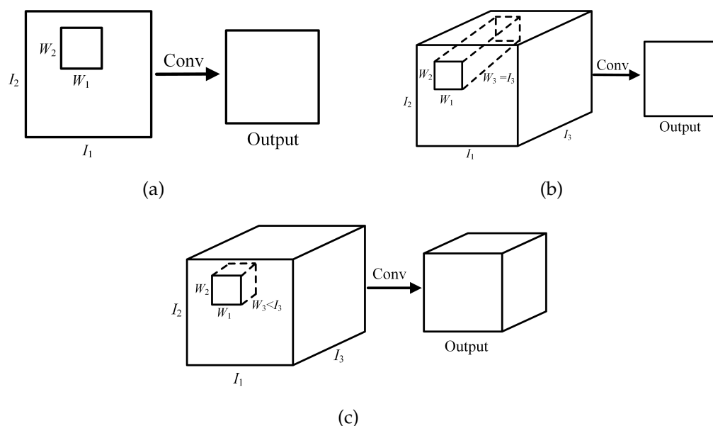
Figure 1. Convolution operation: (a) 2D convolution for a single-channel, (b) 2D convolution for multi-channel, (c) 3D convolution.
