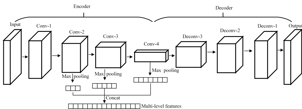
Figure 3. The proposed framework for multi-level feature extraction.
