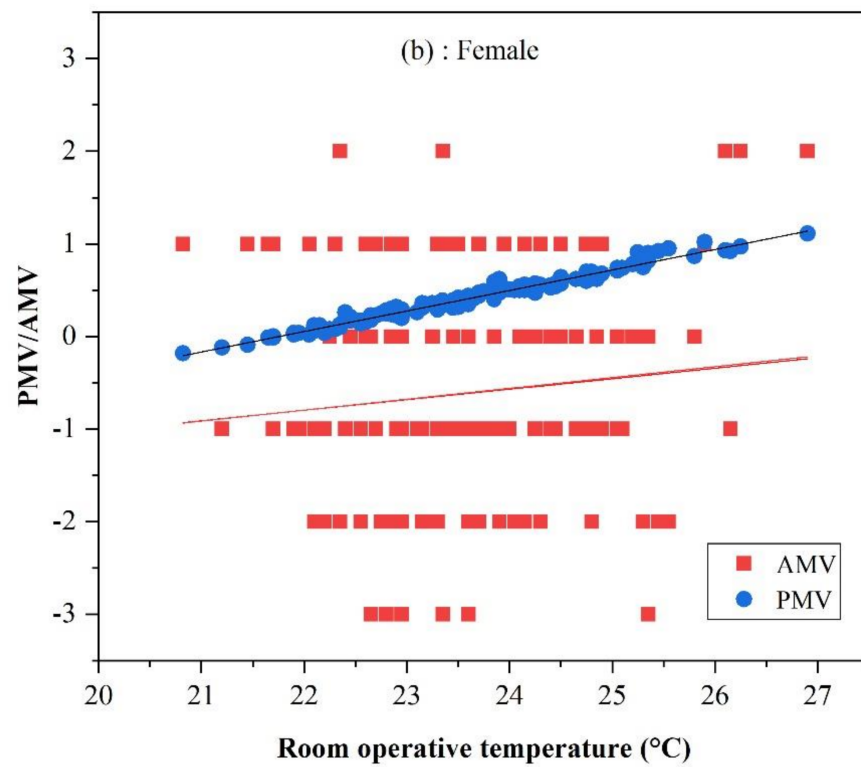
Figure 9. Comparison between actual mean vote (AMV) and predicted mean vote (PMV) versus operative temperature for (a) male and (b) female patients.
