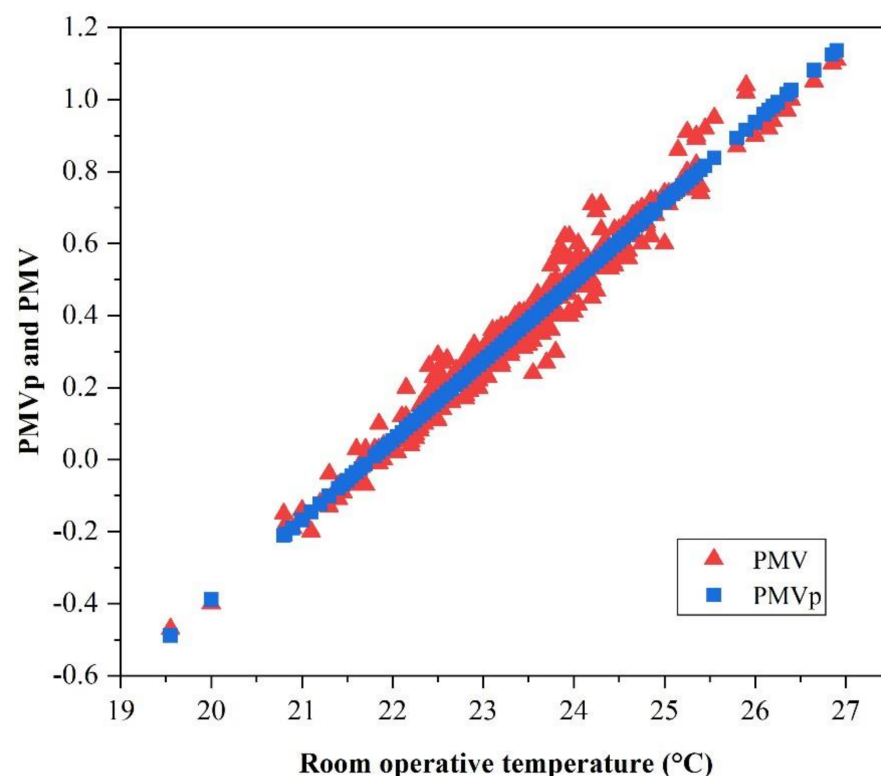
Figure 17. Predicted mean vote for patients (PMV p ) and predicted mean vote (PMV) as a function of operative temperature.
