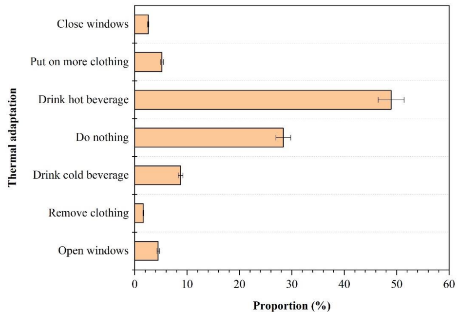
Figure 12. Proportion of patients' adaptive responses.
