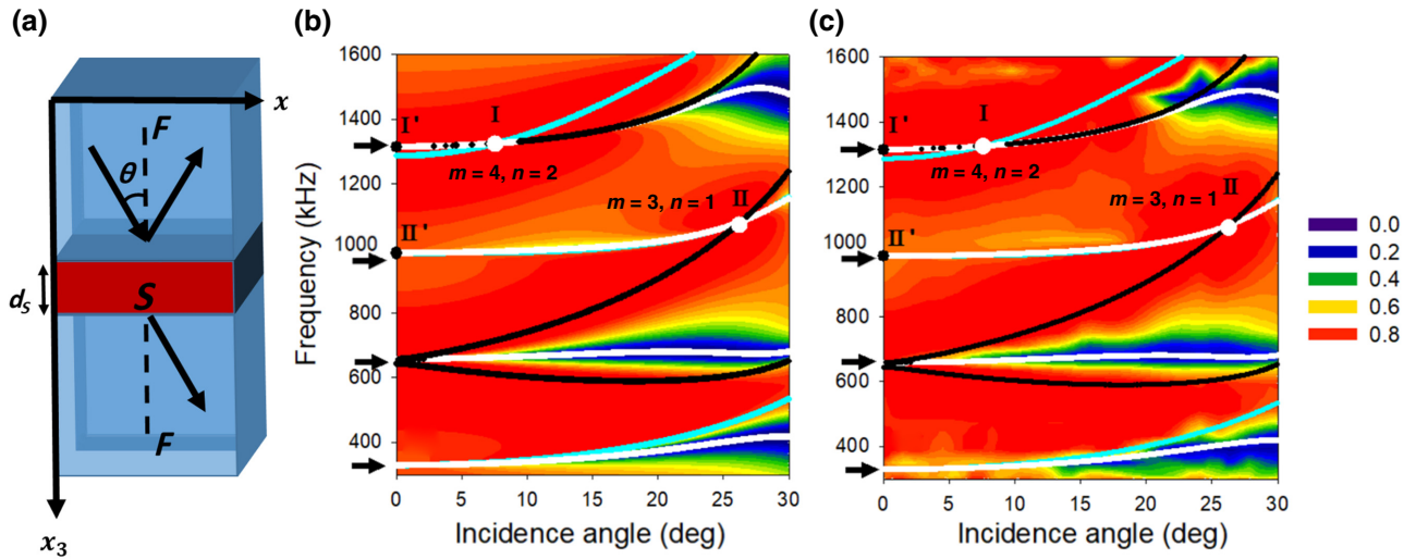
FIG. 1. (a) Schematic representation of a solid layer S (plexiglass) of thickness d_S sandwiched between two semi-infinite liquids F (water). Here \theta is the angle of incidence. (b) Theoretical and (c) experimental variation of transmission versus the frequency and the angle of incidence. White dotted curves represent the frequencies of the transmission zeros (total reflection), whereas black and cyan curves are associated with symmetric and antisymmetric modes of the solid layer with free surfaces, respectively. The latter theoretical curves are added on top of the experimental results for the sake of discussion. The black arrows at the normal incidence indicate the positions of the SP BICs.
