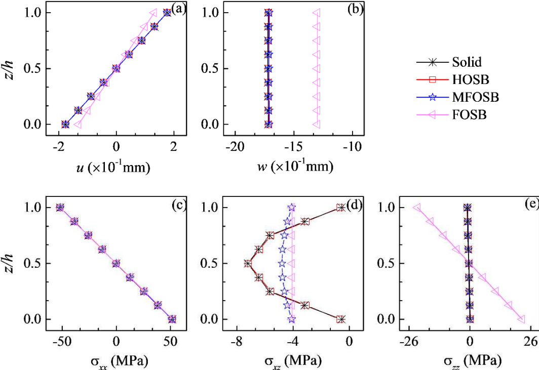
Fig. 8. Straight beam with square cross-section under distributed loading – Through-the-thickness displacement and stresses along a line JK , in the thin case.
