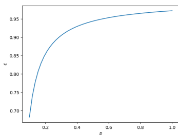
Fig. 4: Privacy parameter \varepsilon of the p -mix M for \delta = 0.01 .
