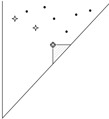
Figure 6: Records in a planar Poisson process above the diagonal t = x of the positive quadrant; ✧ - record (no Poisson atoms south-west of it), ⊛ - the last record (its box contains no Poisson atoms).
