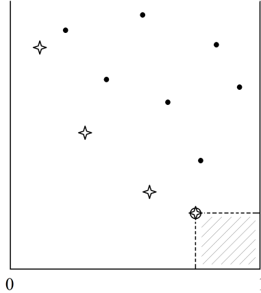
Figure 1: Records in a planar Poisson process in [0, 1] \times [0, \infty) ; ✧ - record (no Poisson atoms south-west of it), ⊕ - the last record (its box contains no Poisson atoms).
