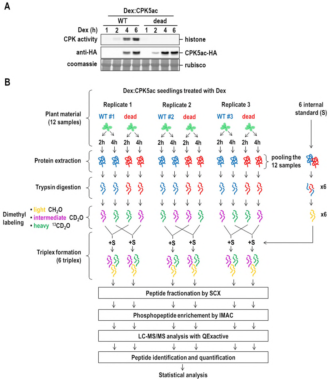
Figure 3. Workflow of the phosphoproteome analysis.
