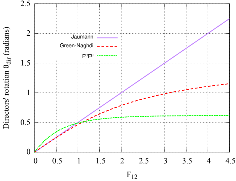
Figure 16: The spin of material directors in the case of a simple glide loading for three different finite strain formulations of crystal plasticity: Jaumann and Green-Naghdi rates and the multiplicative decomposition
