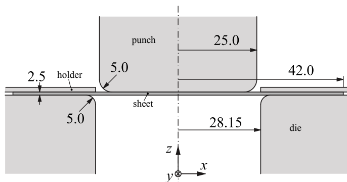
Figure 18: Schematic view of the cup drawing process. No friction is considered between sheet and tools. The die, punch and the holder are assumed to be linear elastic with a Young modulus of E = 10^6 MPa and a Poisson ratio \nu = 0.3 . Lengths in mm.
