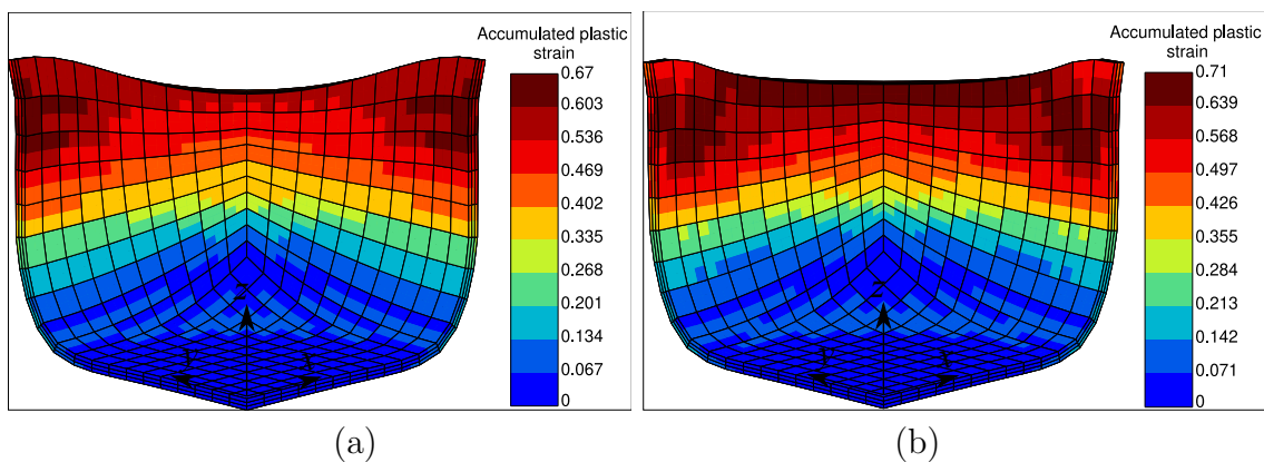
Figure 19: Accumulated plastic strain induced by cup drawing in an anisotropic elastoplastic plate: (a) Without plastic spin \beta = 0 MPa ^{-1} , (b) with plastic spin \beta = 0.01 MPa ^{-1}
