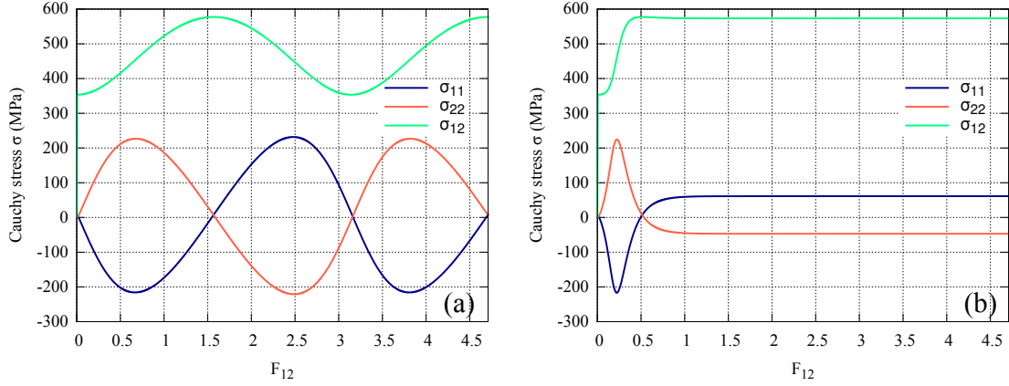
Figure 13: Effect of plastic spin on stress values in the case of simple glide loading. (a) Without plastic spin i.e. \beta = 0 \text{ MPa}^{-1} (b) with plastic spin \beta = 0.01 \text{ MPa}^{-1} . Multiplicative plasticity model with yield stress R_0 = 1000 \text{ MPa} , Hill yield criterion coefficients F = G = H = 0.5 , L = M = 1.5 , N = 4 .
