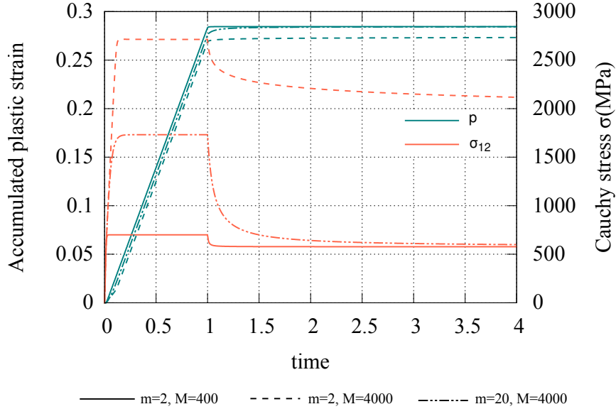
Figure 9: Relaxation test: Higher values of m and lower values of M result in a faster recovery of kinematic hardening. C = 300000 MPa, D = 20 . Parameter M in MPa.
