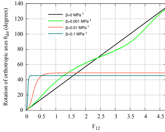
Figure 14: Directors' spin for various values of parameter \beta during a simple glide test for a Hill perfectly plastic material and multiplicative decomposition. When \beta = 0 \text{ MPa}^{-1} , the rotation rate of directors is constant and coincides with the material spin.
