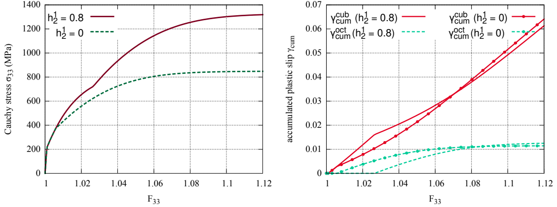
Figure 17: A single crystal including two slip system families (octahedral and cubic) in tension along \langle 111 \rangle . \gamma_{cum}^{cub} (resp. \gamma_{cum}^{oct} ) denotes the accumulated cubic (resp. octahedral) plastic slip.
