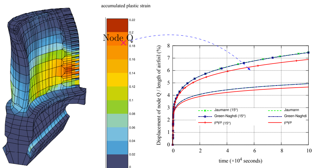
Figure 21: (a) The accumulated plastic strain in a turbine blade subjected to creep at high temperature. (b) Displacement of the node Q as a function of time: comparison of different finite deformation formulations.
