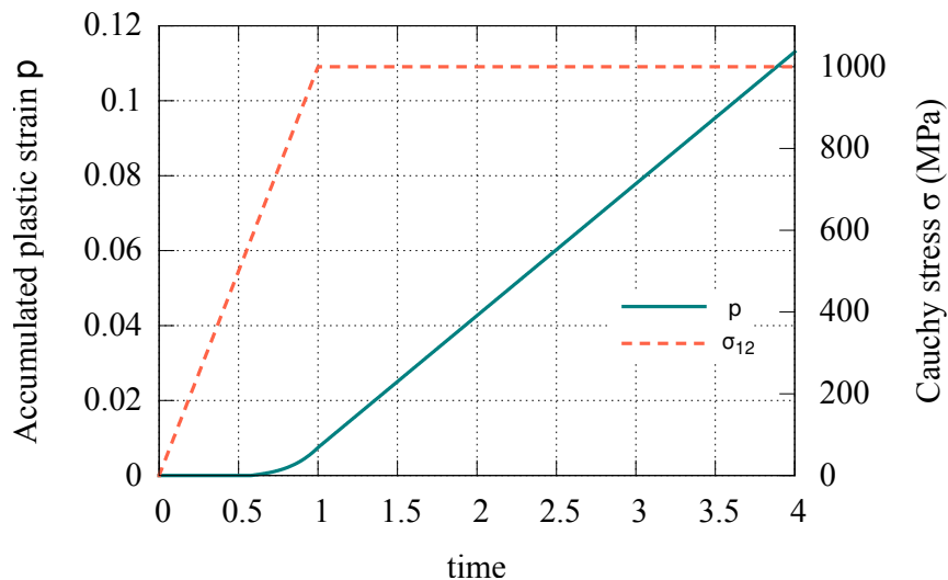
Figure 10: Plastic flow during a creep test.
