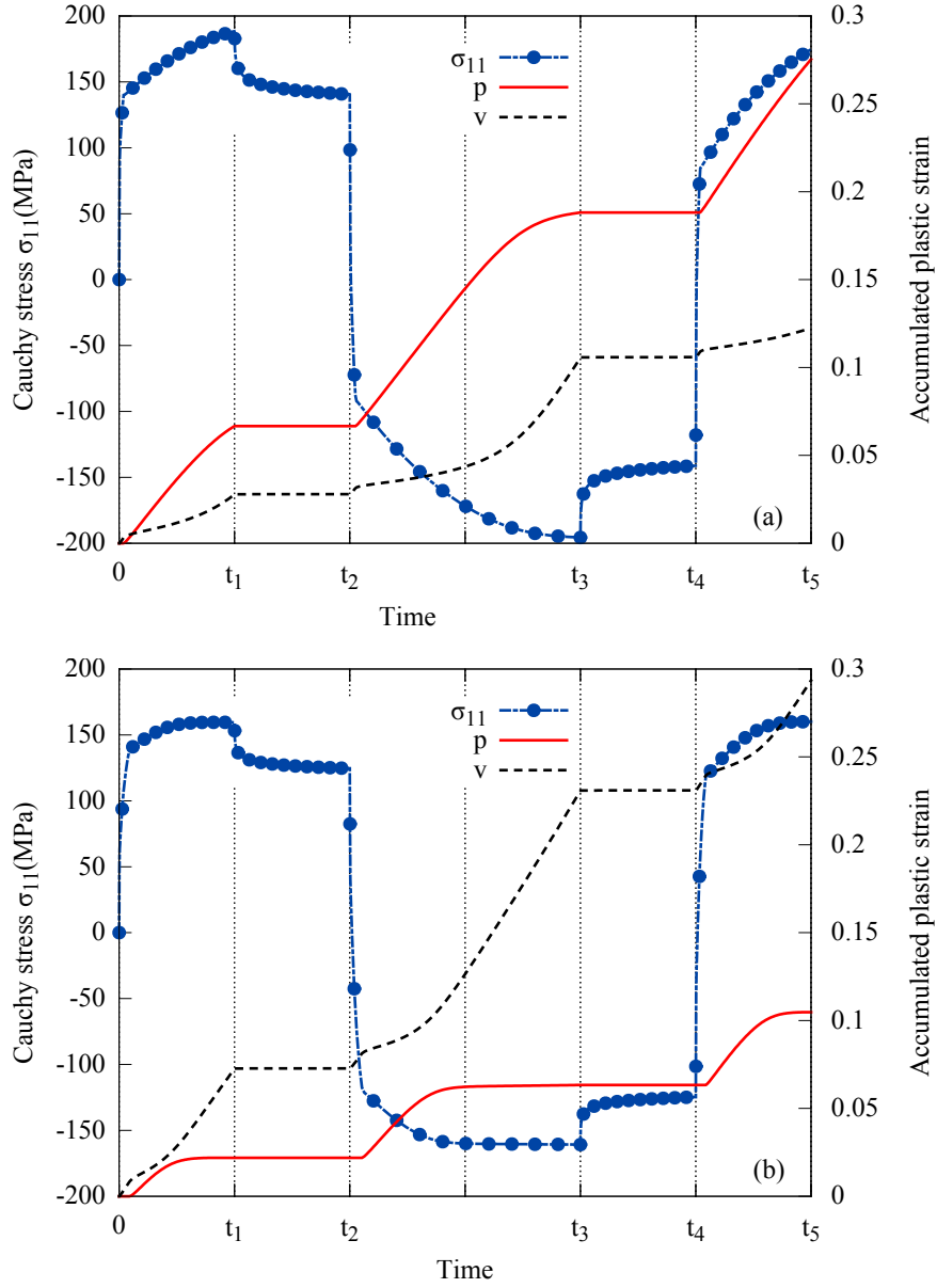
Figure 11: Tension/compression test for two deformation rates \dot{F}_{11} = 0.1 \text{ s}^{-1} (a) and \dot{F}_{11} = 0.001 \text{ s}^{-1} (b). Model with a time-independent and a viscoplastic mechanism.
