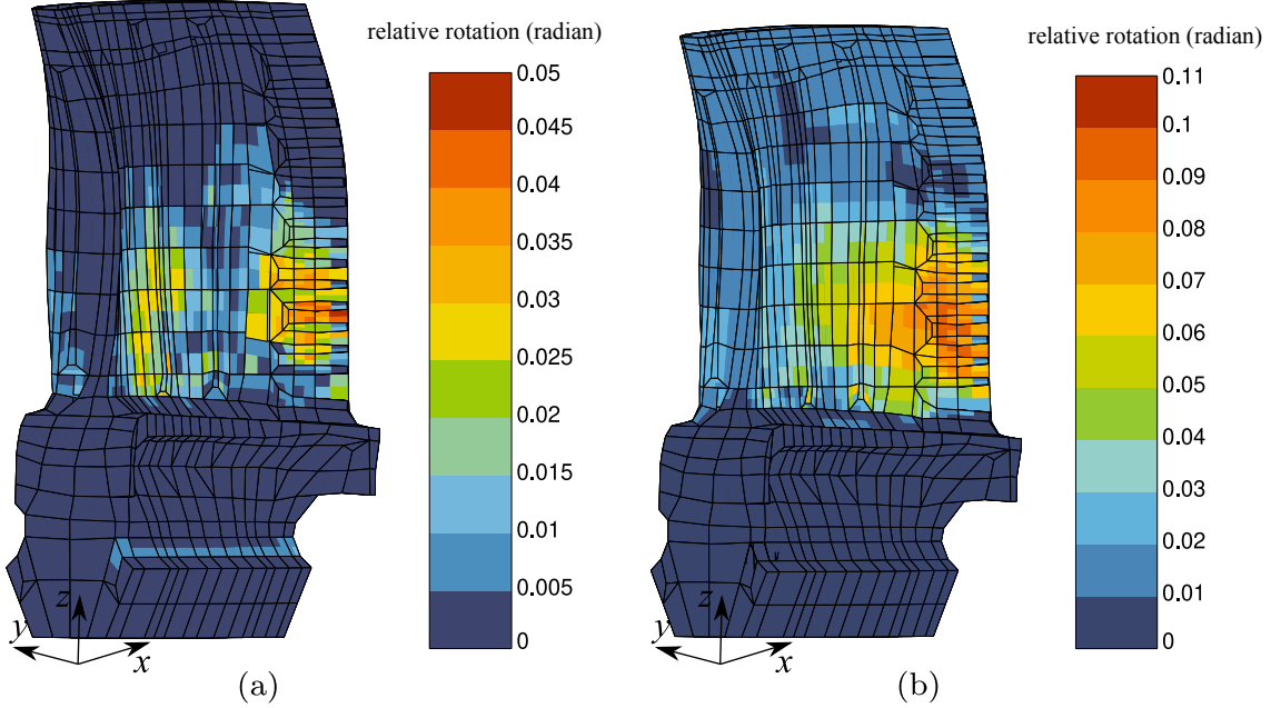
Figure 22: Relative rotation of crystal directors w.r.t. material lines for the multiplicative-based model in two cases (a) ideal \langle 1001 \rangle orientation of the blade, (b) deviation of 15^\circ around y-axis.
