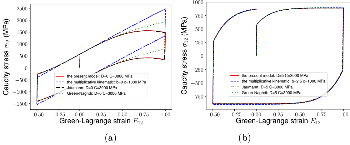
Figure 8: Cyclic simple glide loading: (a) linear ( D = 0 ) (b) nonlinear kinematic hardening with dynamic recovery.
