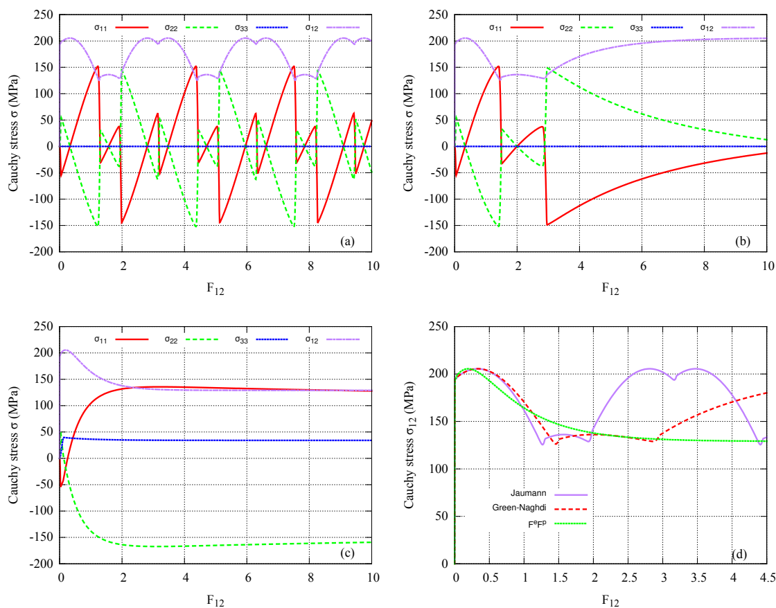
Figure 15: The effect of plastic spin in the case of a simple glide loading of a FCC single crystal for three different finite strain formulations: Jaumann (a) and Green-Naghdi(b) rates (with no plastic spin) and the multiplicative decomposition (c). (d) comparison of \sigma_{12} for all three formulations.
