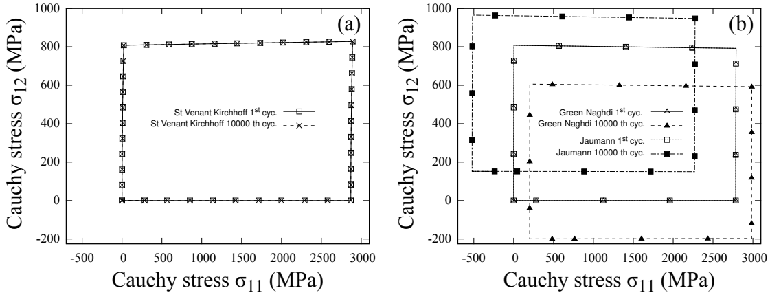
Figure 5: Case 1, the resulting stress during the first and the 10000th cycles for (a) hyperelastic material (b) hypoelastic materials. Young's modulus E = 210000 MPa, and Poisson ratio \nu = 0.3 .
