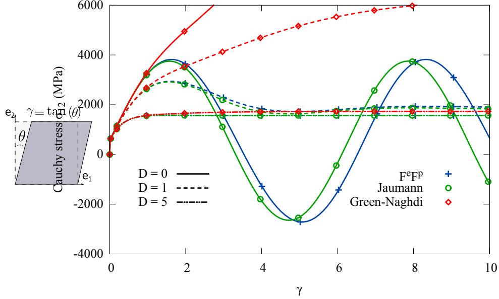
Figure 7: Monotonic simple glide test for different formulations of elastoplasticity with kinematic hardening: Stress oscillations in the case of Jaumann rate and the multiplicative decomposition if D = 0 . These oscillations are suppressed as the parameter D increases. Values of material parameters: C = 10000 MPa, R_0 = 1000 MPa.
