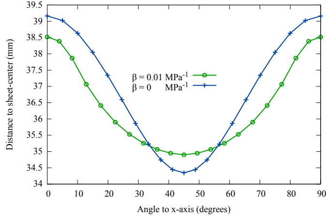
Figure 20: Distance of rim to the sheet center versus angle to x-axis. The curve shows the earing pattern for two values of the parameter \beta .
