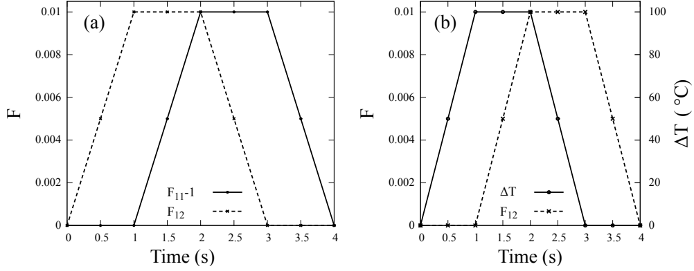
Figure 4: Illustration of loading conditions corresponding to (a) case 1, (b) case 2
