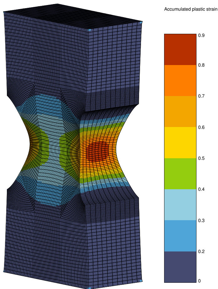
Figure 23: Accumulated plastic strain in a notched specimen subjected to tensile loading using the multiplicative decomposition based model.
