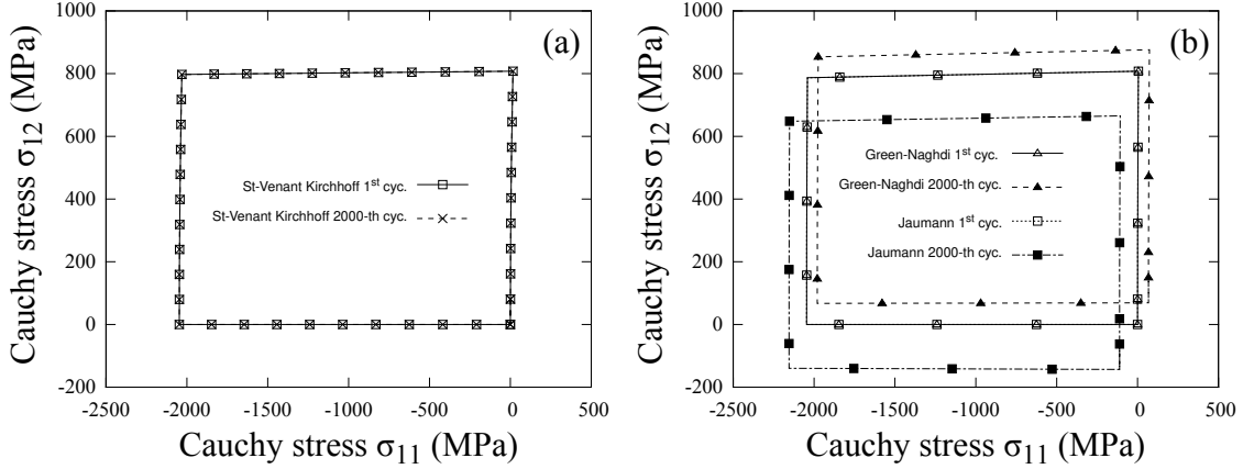
Figure 6: Case 2, the resulting stress during the first and the 2000th cycles for (a) hyperelastic material (b) hypoelastic materials. E = 210000 MPa, \nu = 0.3 and \alpha_T = 10^{-4} K^{-1}
