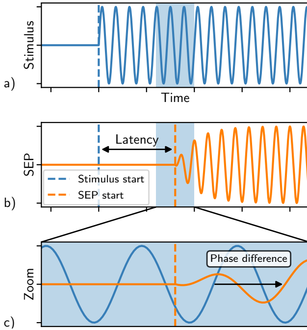
Figure 3. Temporal characteristics of an theoretical SEP reaching its steady-state. (a) The “stimulus” plot is the representation of the periodical somatosensory stimulus amplitude vs. time, considered here as a windowed sine function. (b) Representation of an ideal SEP elicited by the stimulus, i.e. an amplitude modulated sine function without noise. (c) Zoom on the plots (a) and (b) around the beginning of the SEP. It shows the phase difference between the SEP and the stimulus.
